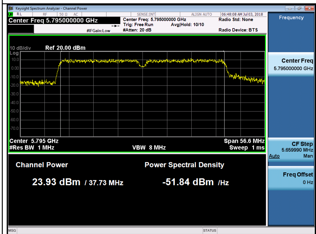
64QAM-5795MHz
