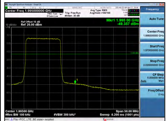
BandEdge-LTE- Band2-15MHz-64QAM-High
