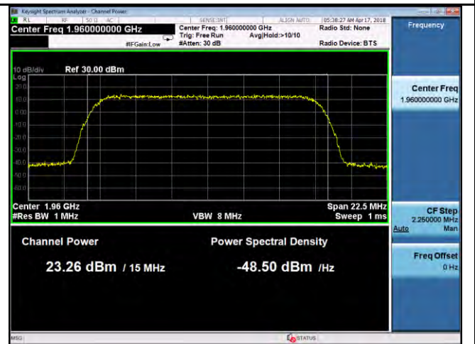
PWR- Band2-QPSK-15M BW-Mid CH-Port2
