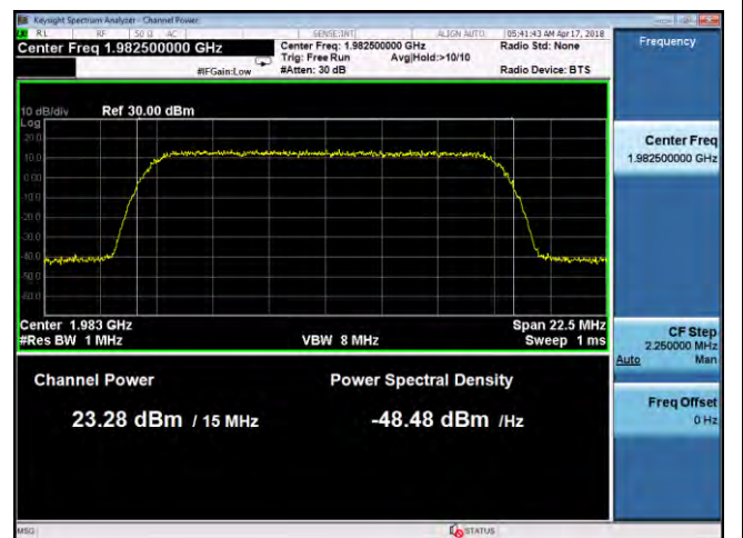
PWR- Band2-QPSK-15M BW-High CH-Port2
