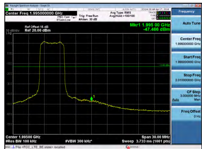
BandEdge-LTE- Band2-5MHz -64QAM-High
