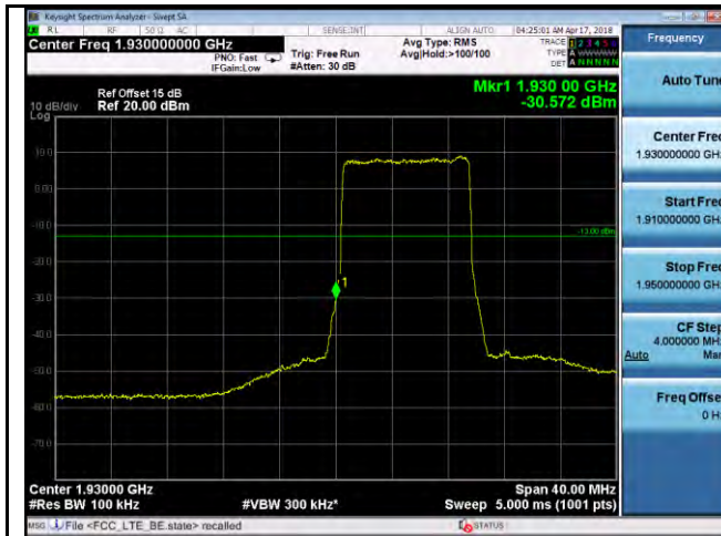
BandEdge-LTE-Band2-10MHz-QPSK-Low
