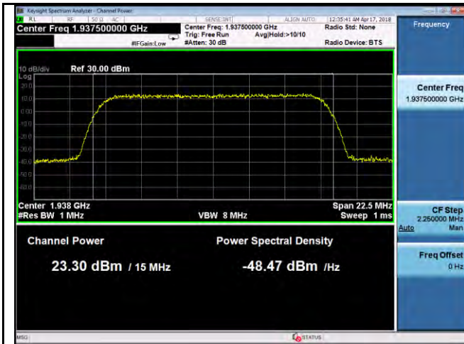
PWR-Band2-QPSK-15M BW-Low CH-Port1
