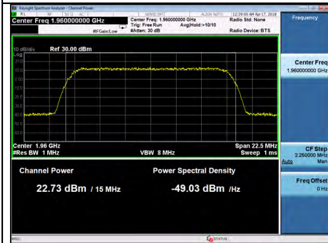
PWR- Band2-QPSK-15M BW-Mid CH-Port1
