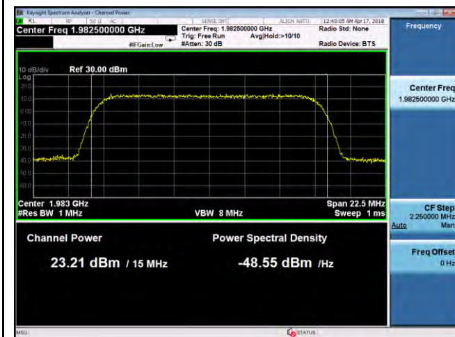
PWR- Band2-QPSK-15M BW-High CH-Port1
