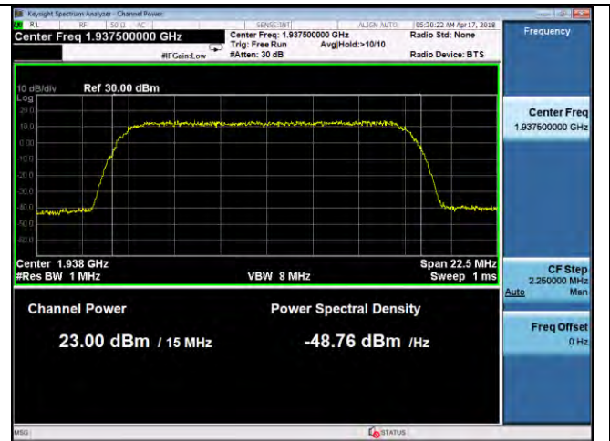
PWR- Band2-QPSK-15M BW-Low CH-Port2
