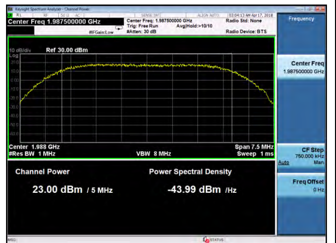
PWR- Band2-64QAM-5M BW-High CH-Port2
