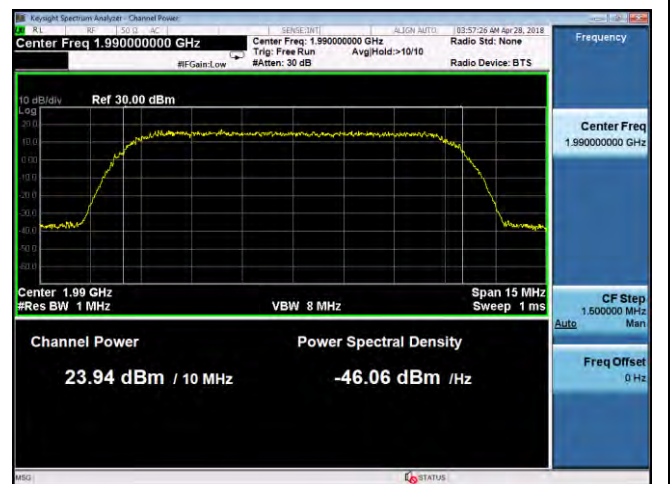
PWR-Band25-QPSK-10M BW-High CH-Port2
