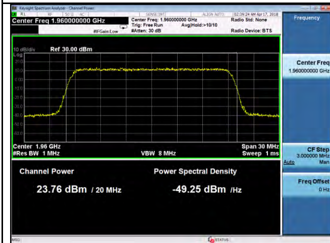
PWR-Band2-64QAM-20M BW-Mid CH-Port1
