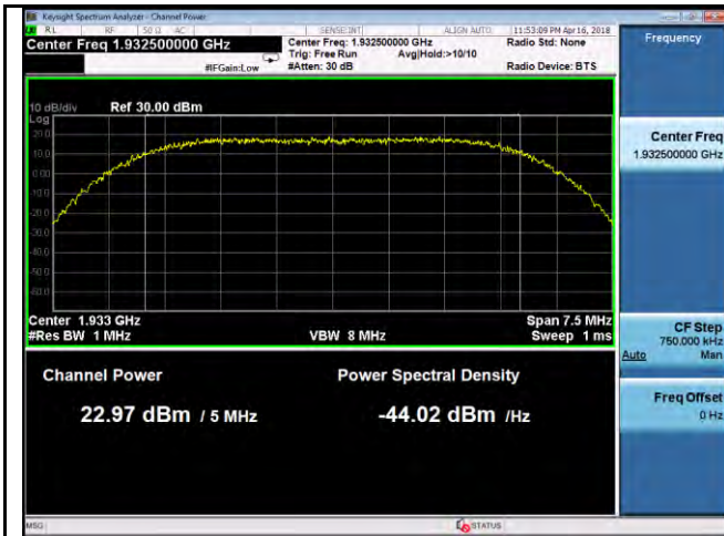
PWR-Band2-64QAM-5M BW-Low CH-Port1
