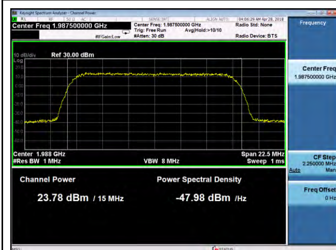
PWR-Band25-64QAM-15M BW-High CH-Port1
