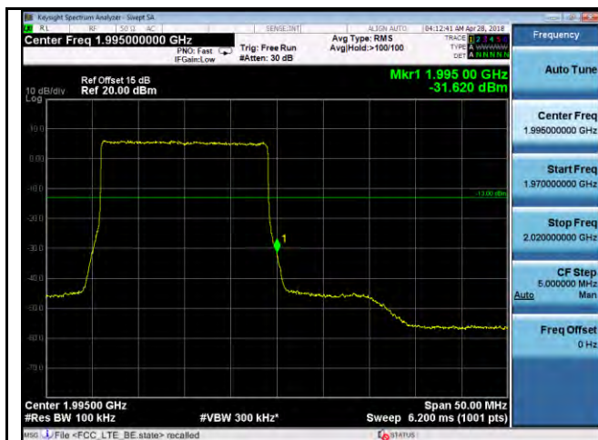
BandEdge-LTE- Band25-20MHz-QPSK-High
