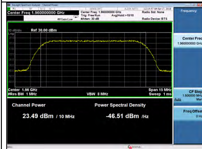
PWR- Band2-QPSK-10M BW-Mid CH-Port1
