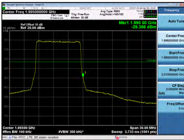
BandEdge-LTE- Band25-10MHz-QPSK-High
