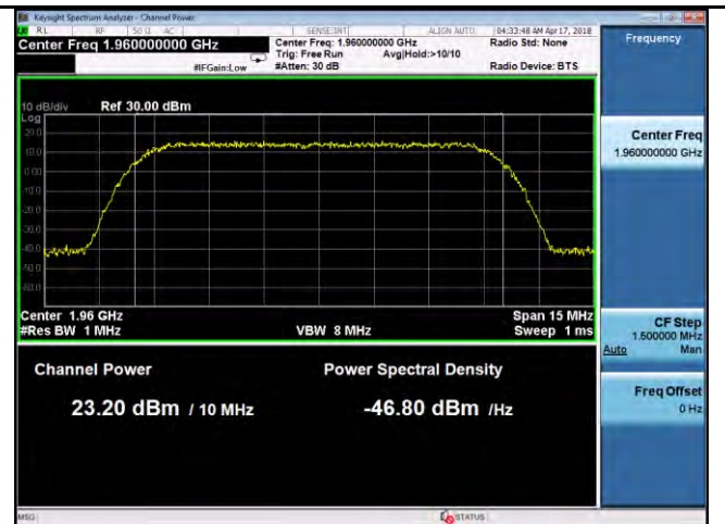
PWR- Band2-QPSK-10M BW-Mid CH-Port2
