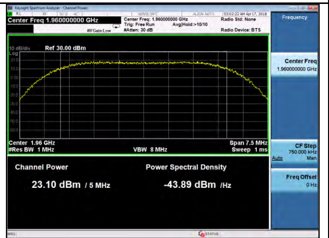
PWR- Band2-64QAM-5M BW-Mid CH-Port2
