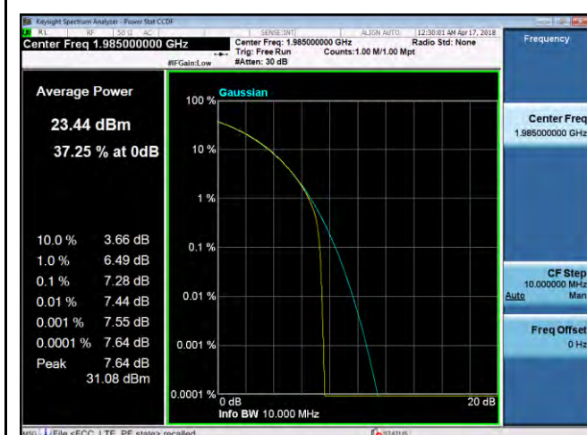
PK-AV-Ratio-Band2-64QAM-10M BW-High
