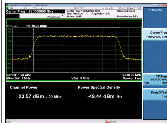
PWR-Band2-64QAM-20M BW-High CH-Port1
