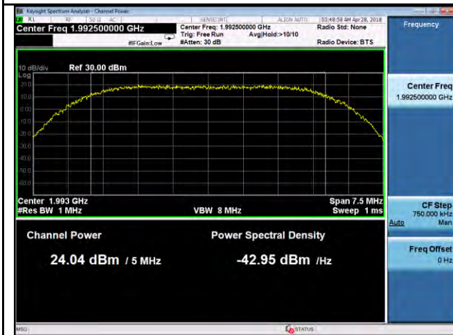
PWR-Band25-64QAM-5M BW-High CH-Port1
