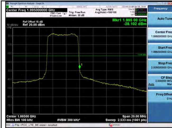
BandEdge-LTE- Band25-5MHz-QPSK-High
