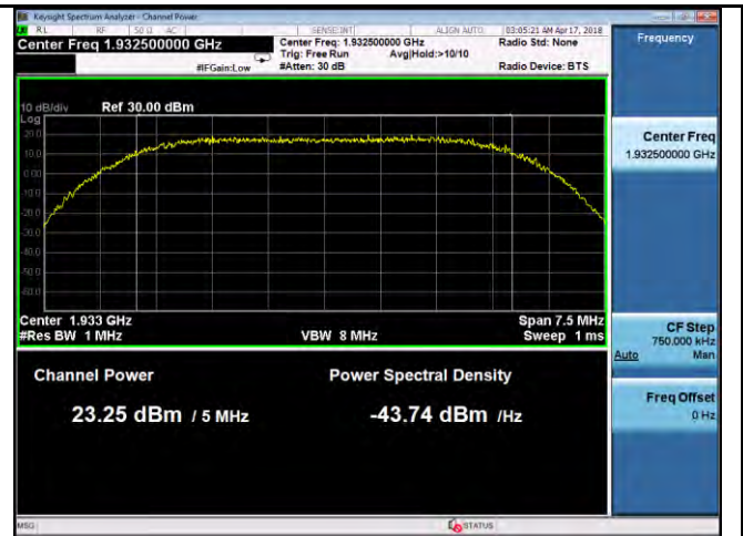
PWR- Band2-64QAM-5M BW-Low CH-Port2
