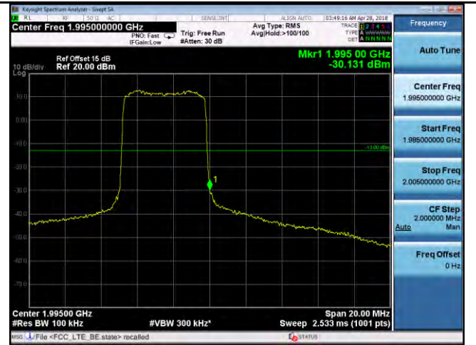
BandEdge-LTE- Band25-5MHz-64QAM-High
