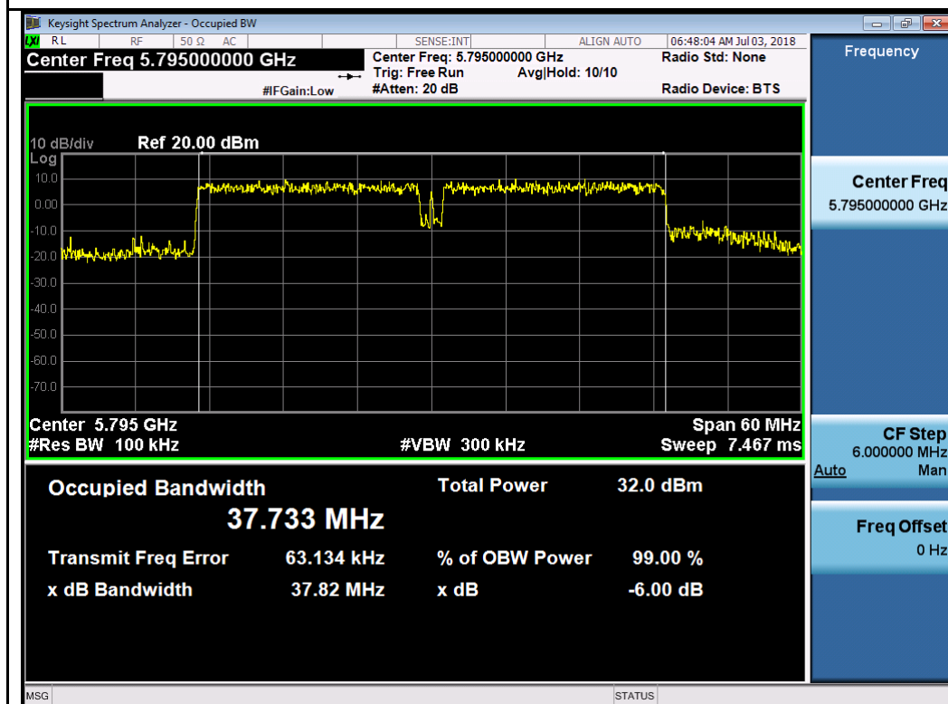
64QAM-5795MHz
