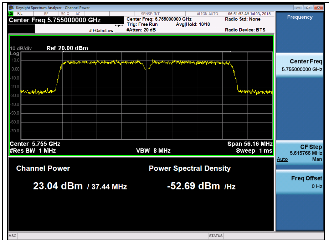
64QAM-5755MHz
