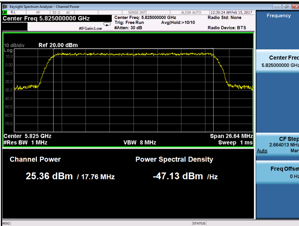
64QAM-5825MHz
