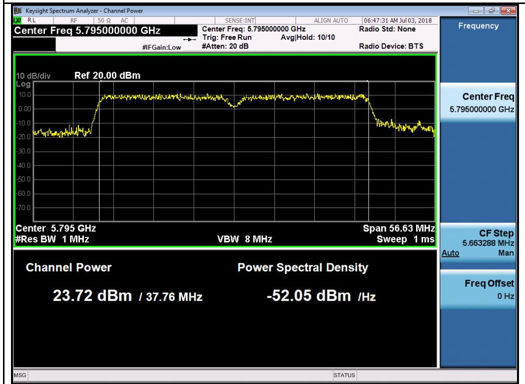
64QAM-5795MHz
