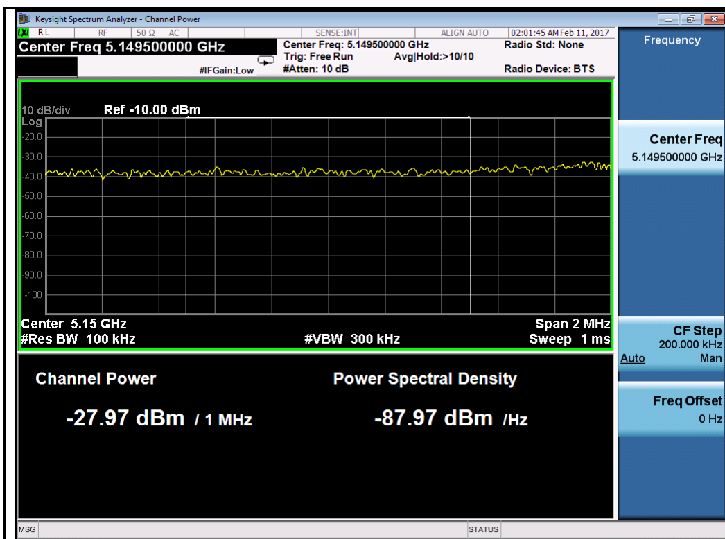
64QAM-5160MHz
