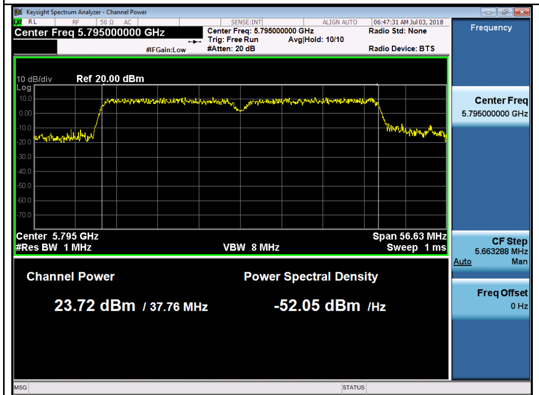
64QAM-5795MHz
