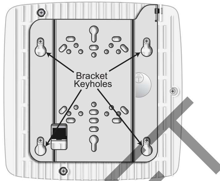
Figure 11 Radio Node Slides into Mount Bracket
