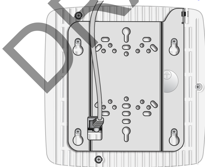
Figure 13 Route and Terminate the Cable
