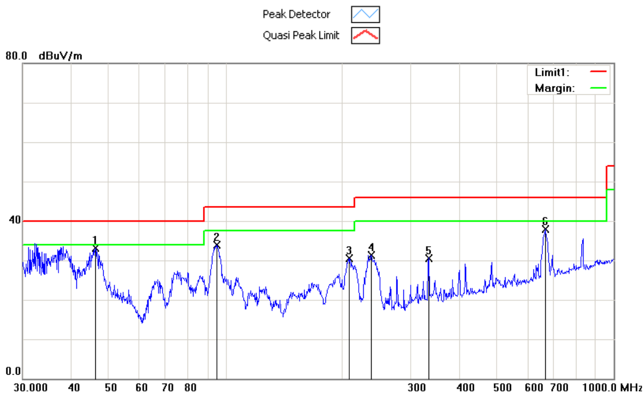
Vertical & Horizontal Polarity Plot @3m
