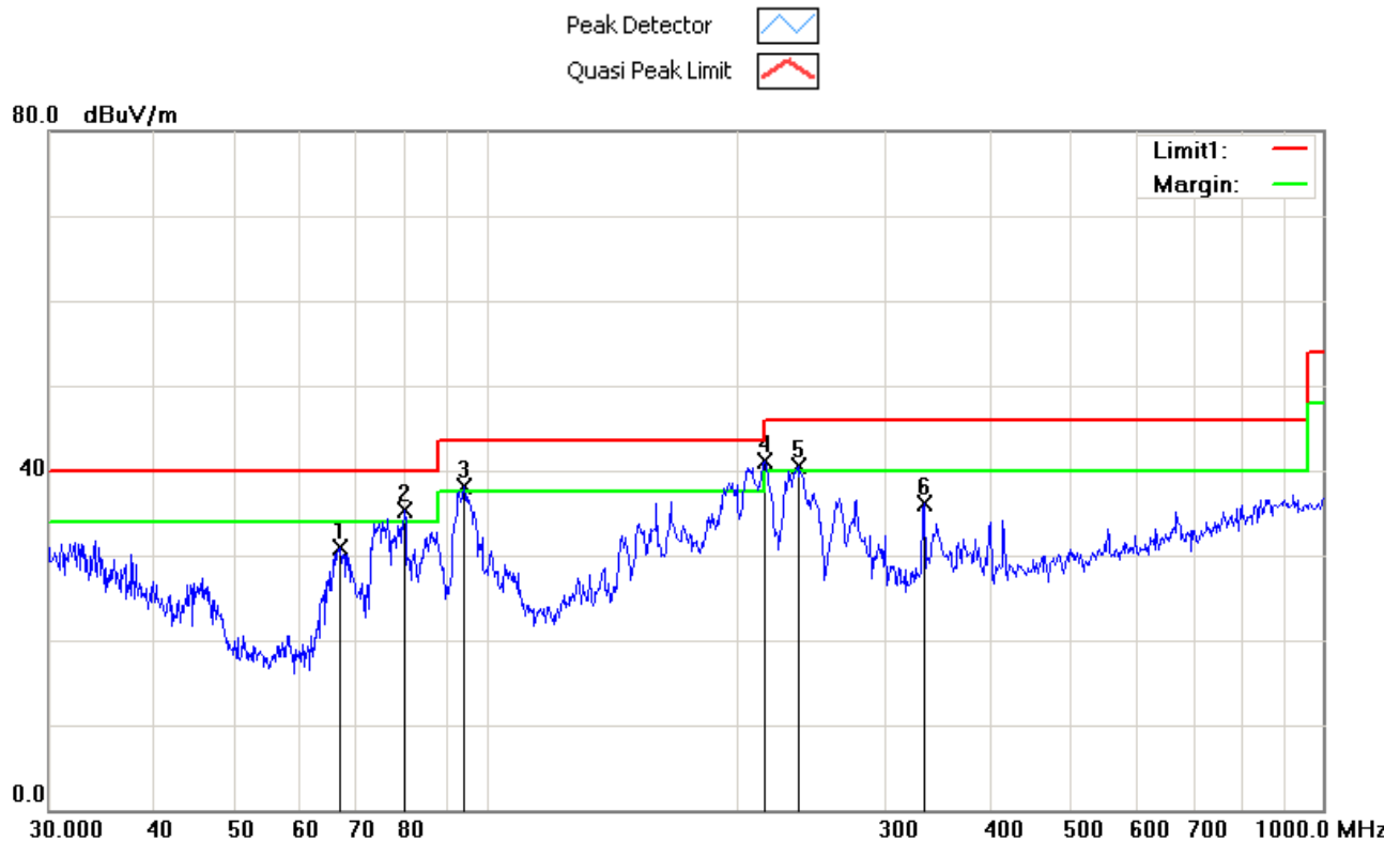
Vertical & Horizontal Polarity Plot @3m
