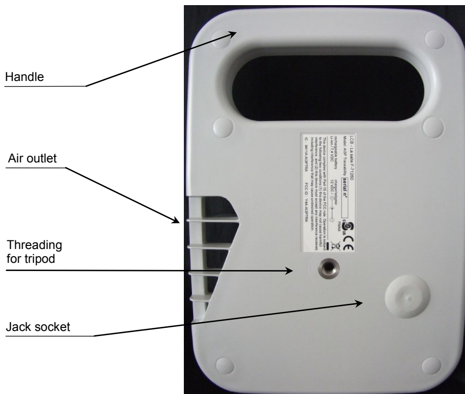
Figure 3-4: Rear face
