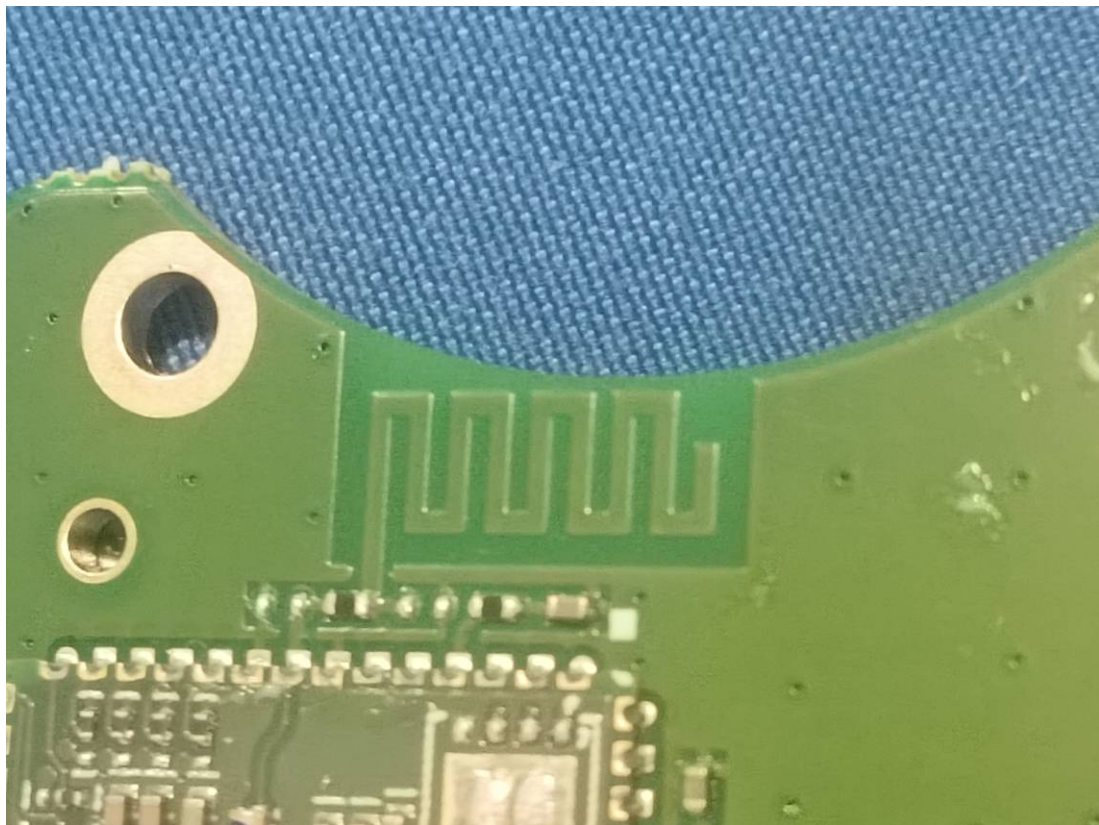
Bluetooth Antenna(DM8000-1)
