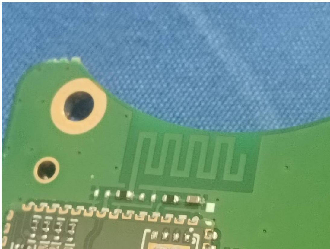
Bluetooth Antenna(DM8100-1)
