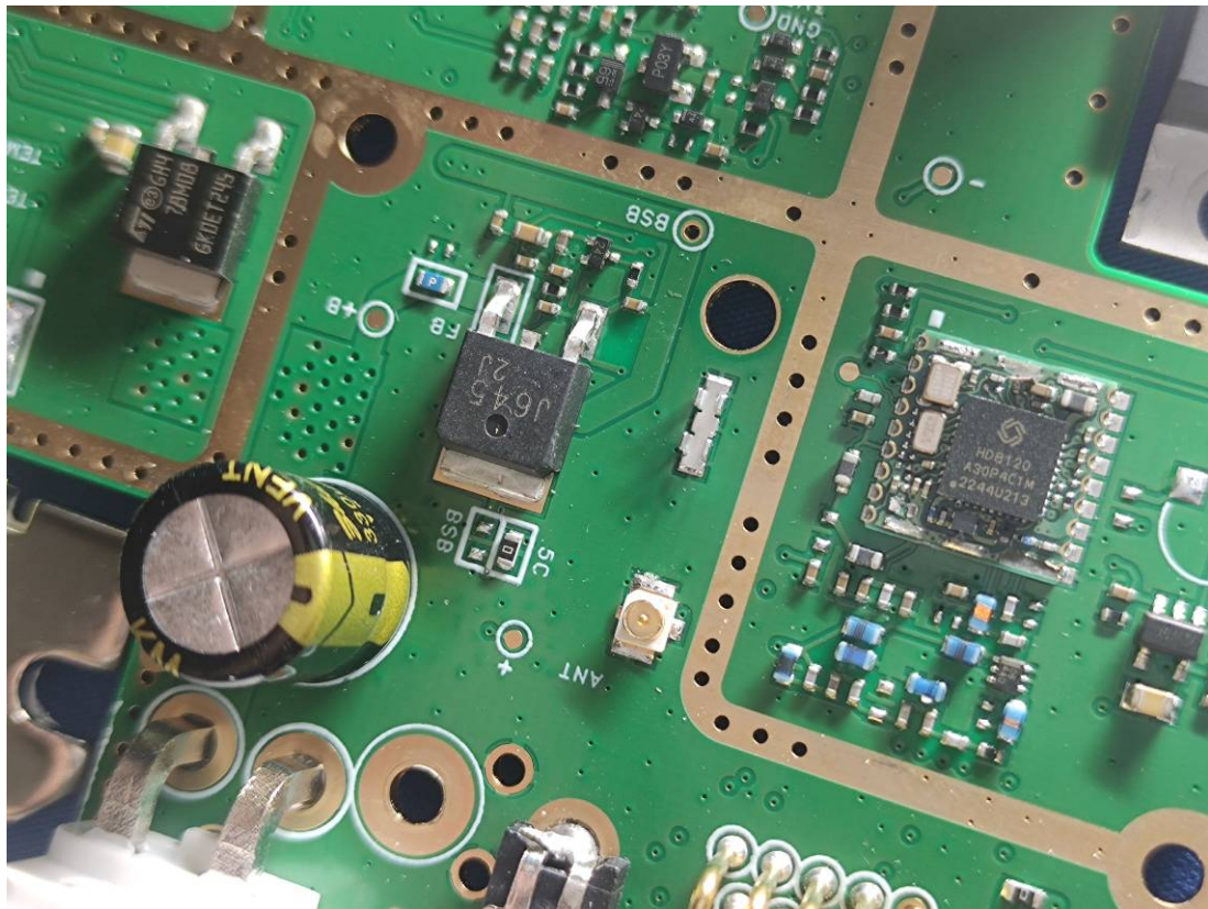
Bluetooth Antenna(DM8000-1)
