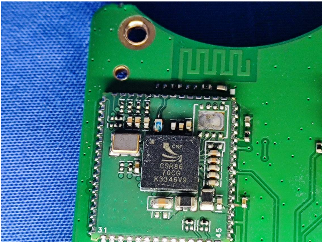
Bluetooth module and Antenna
