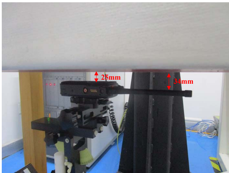
Face Up Setup Photo_ DR7500-1_136-150 MHz(25mm)
