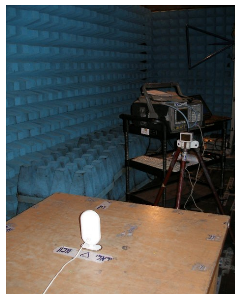
Photo 2. Spurious emissions test setup.
