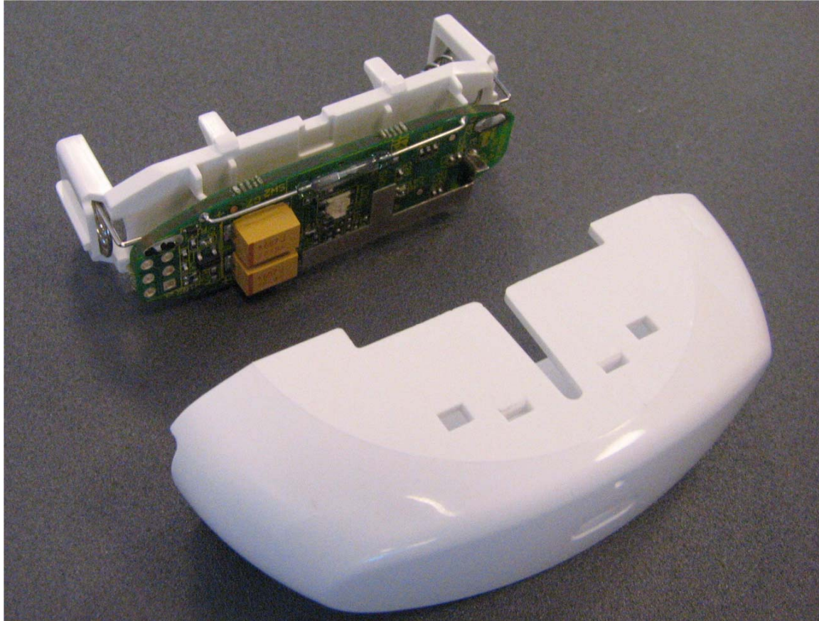
Photograph No.4 M800MGL magnet sensor (detector) with case removed
