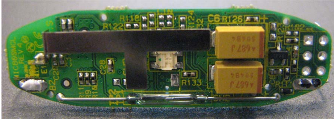
Photograph No.5 M800MGL magnet sensor (detector) PCB front view
