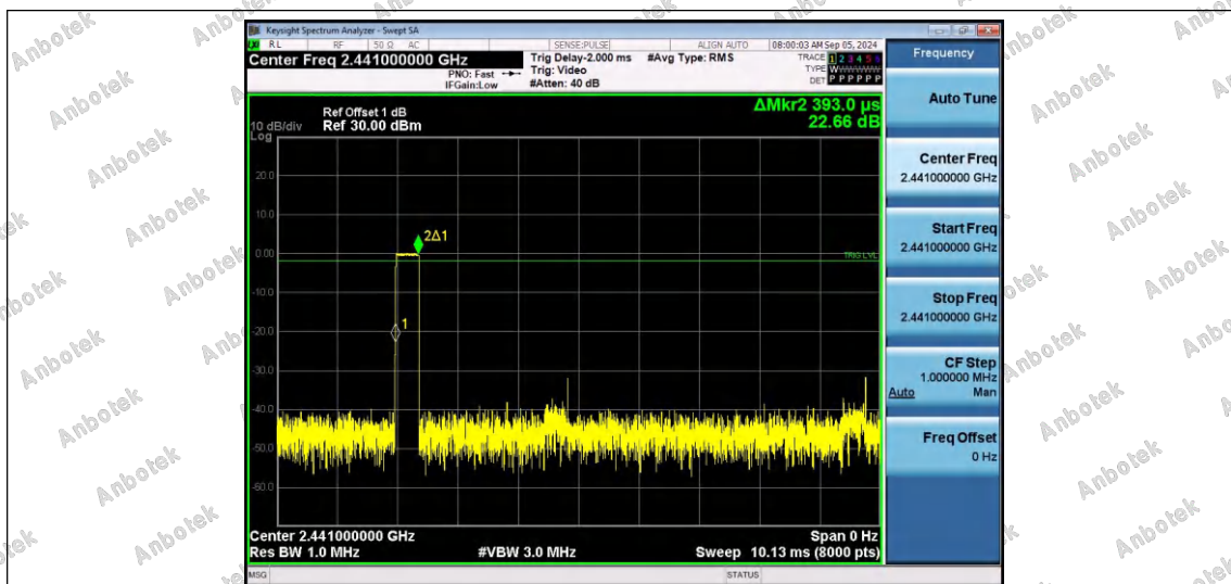
DH1-Ant1-Hop-PASS
