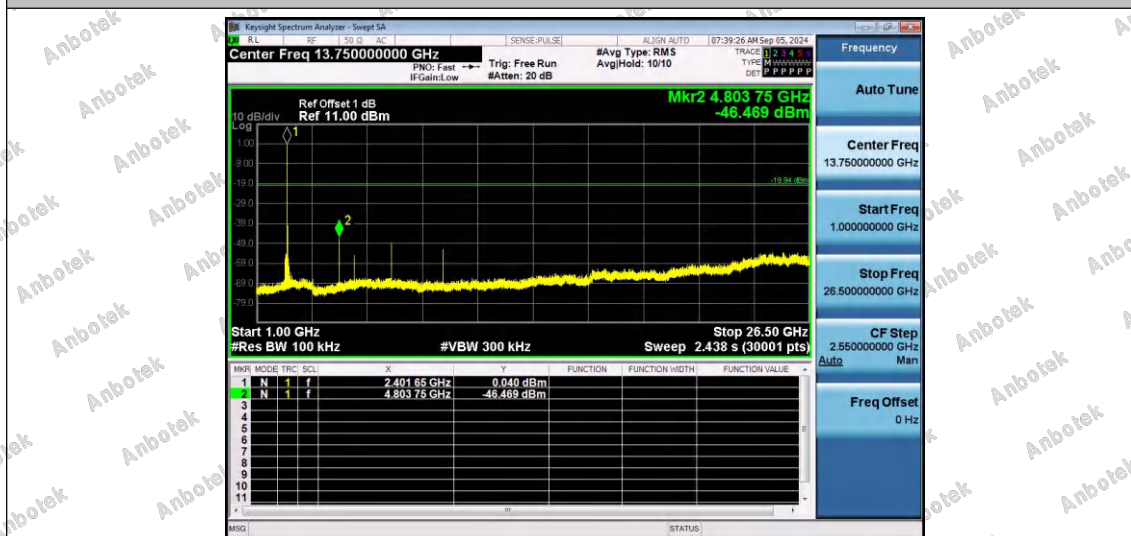
DH5-Ant1-2402-1000~26500-PASS
