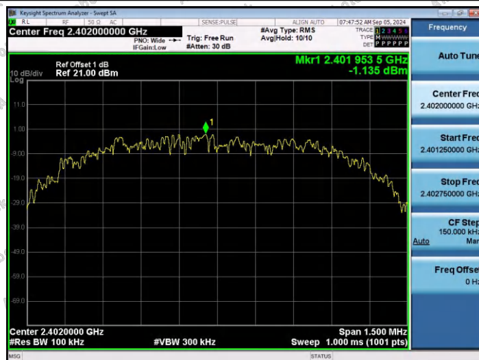
3DH5-Ant1-2402-0~Reference-PASS
