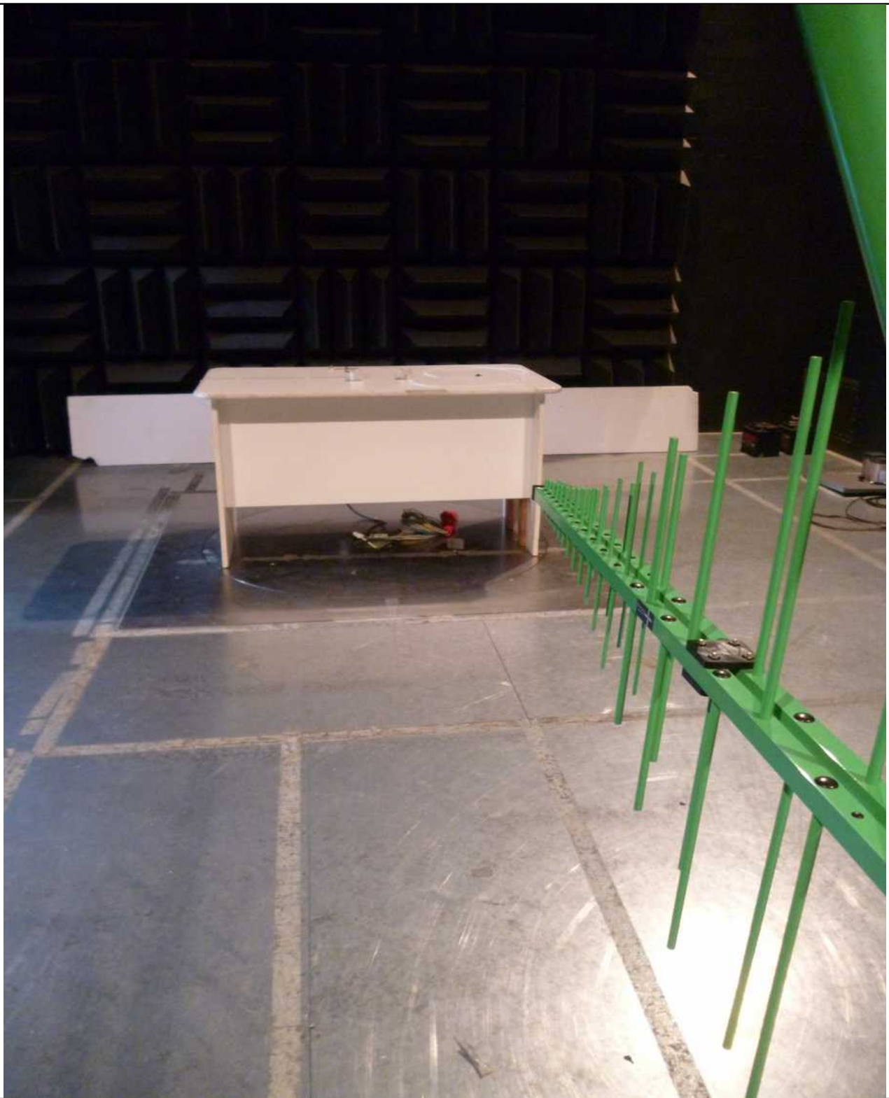
Radiated Emissions Test Set-up
