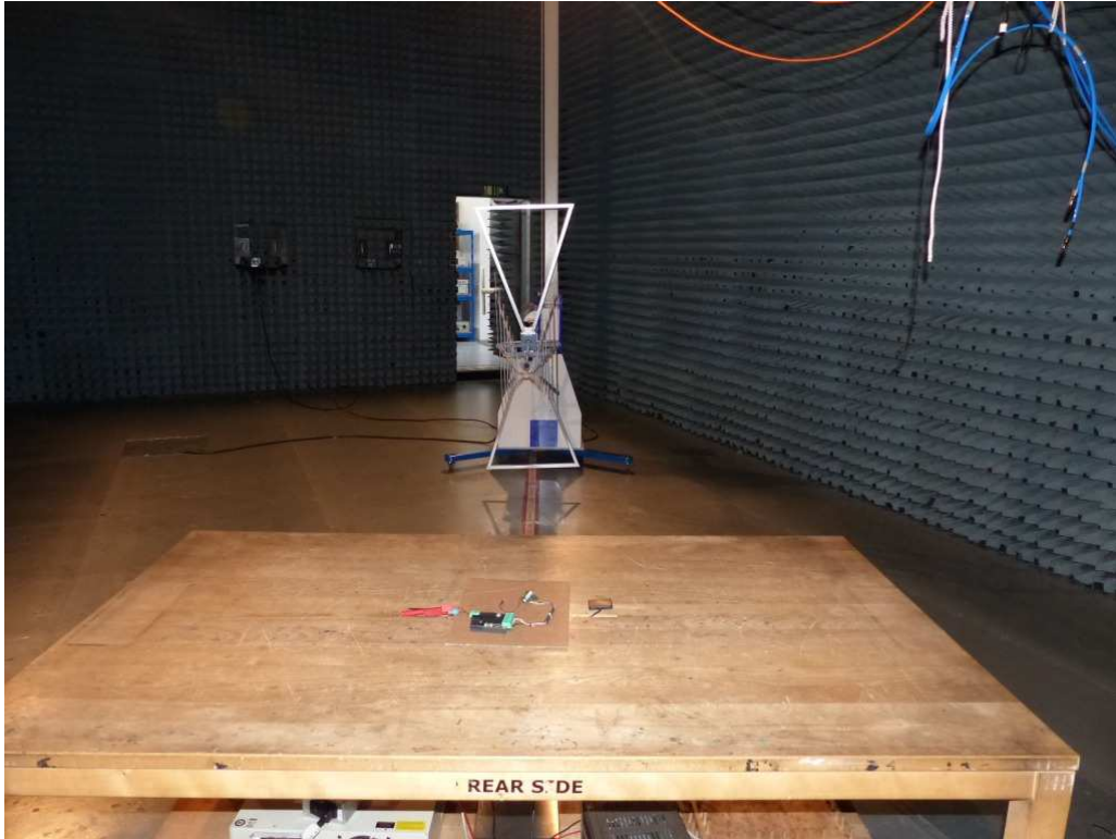
Photo 5: Test setup for radiated measurements (computer peripheral setup, EUT supplied by external DC power to enable USB data transfer to computer, unintentional radiator §15)
