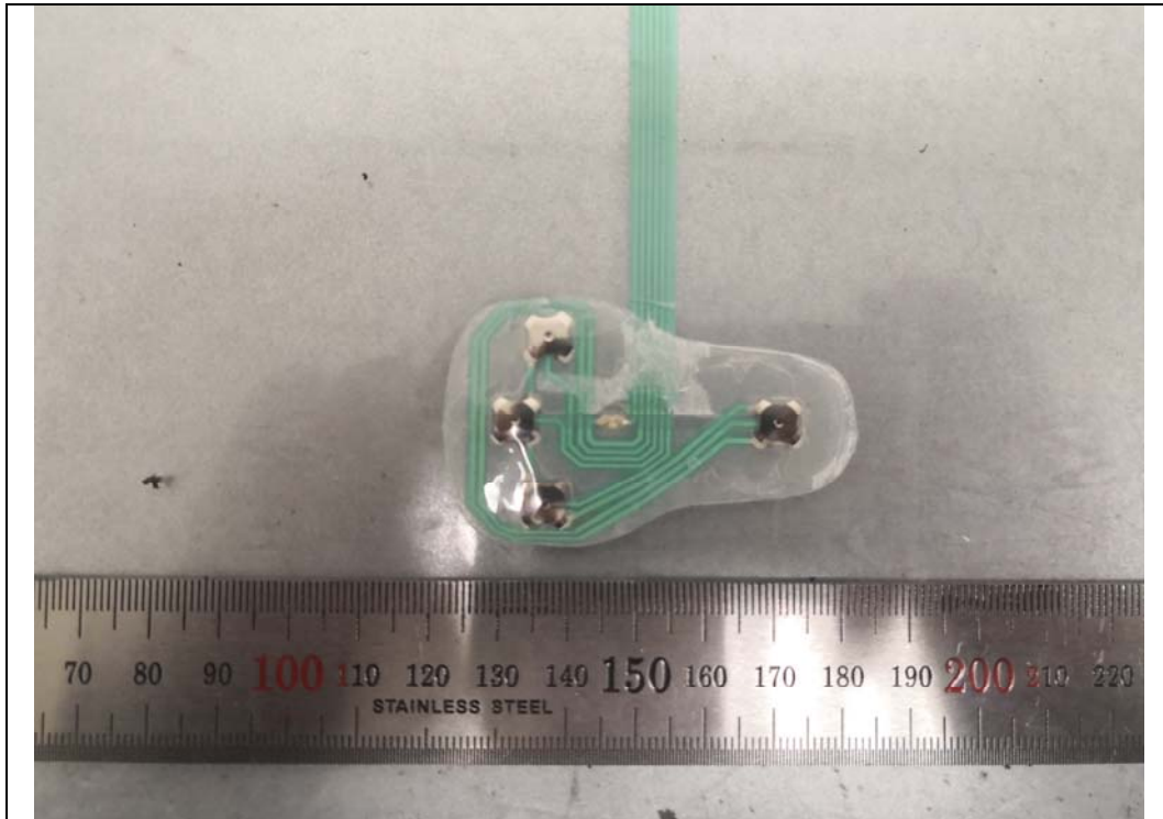
Switch Board Front
