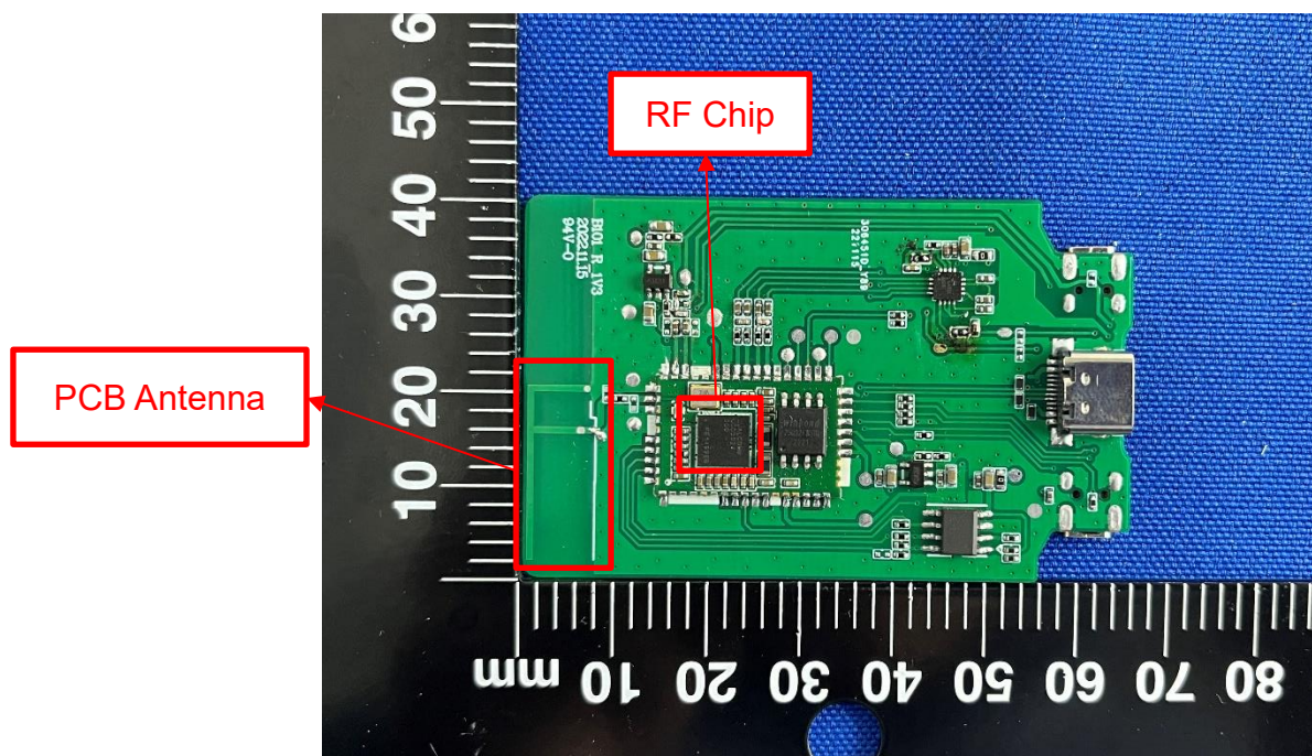
MAIN BOARD TOP VIEW
