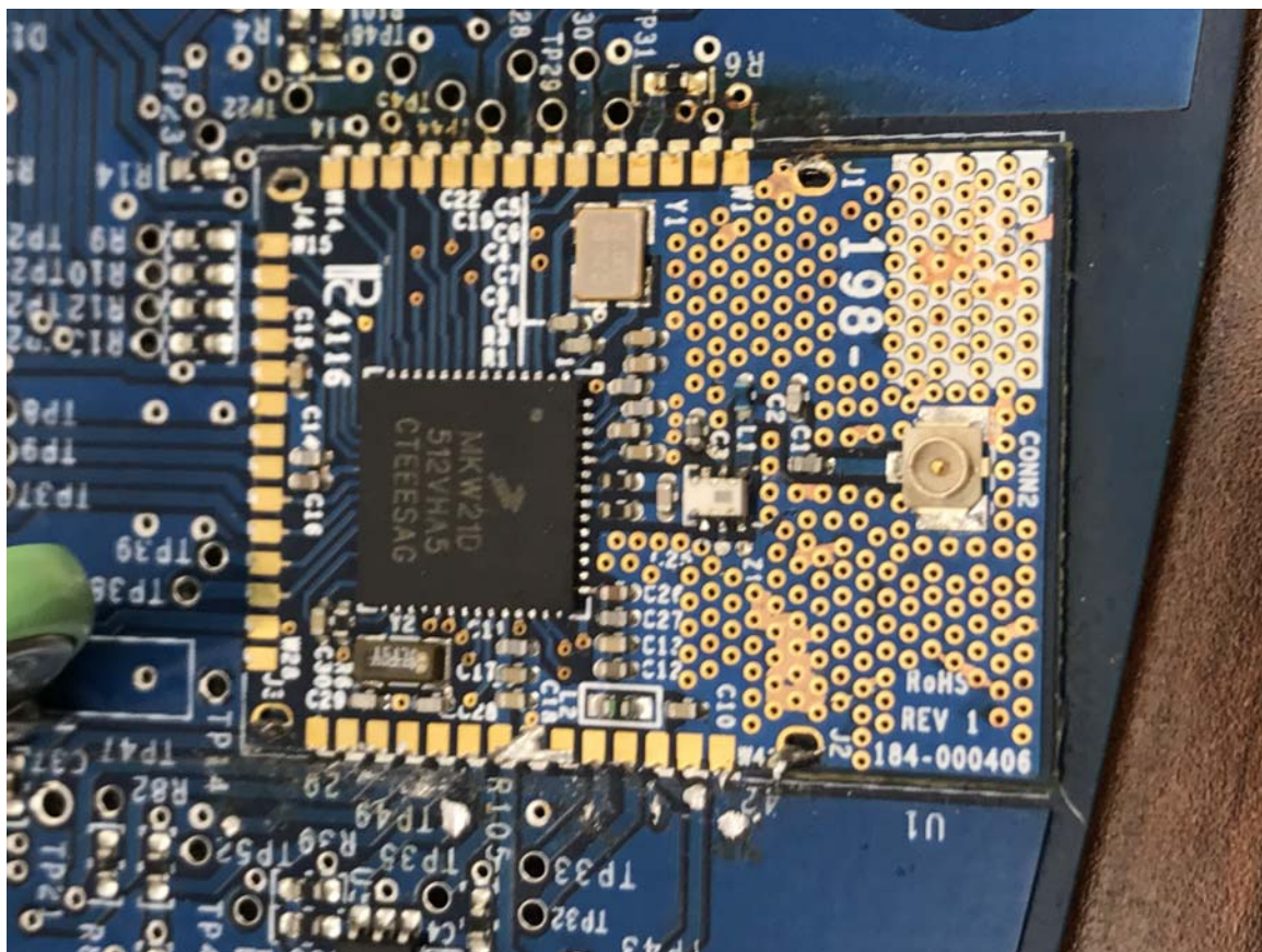
Front of module installed in host; Shield Removed (External Antenna)
