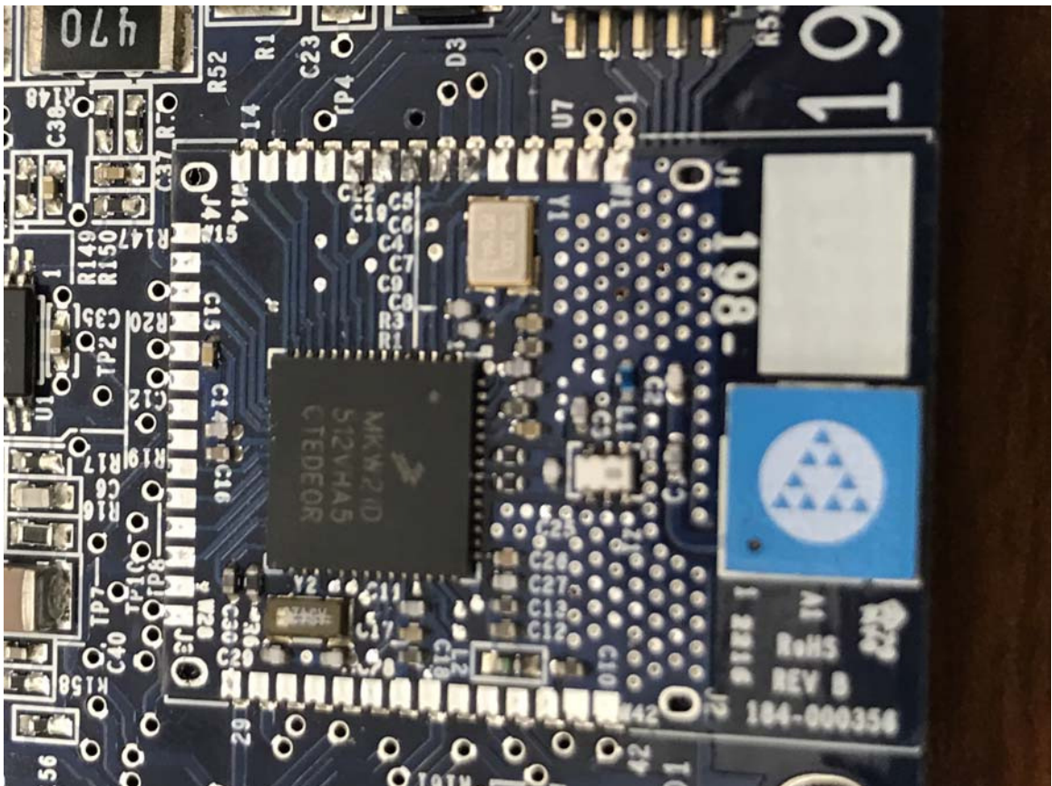
Front of module installed in host; Shield removed (Chip Antenna)
