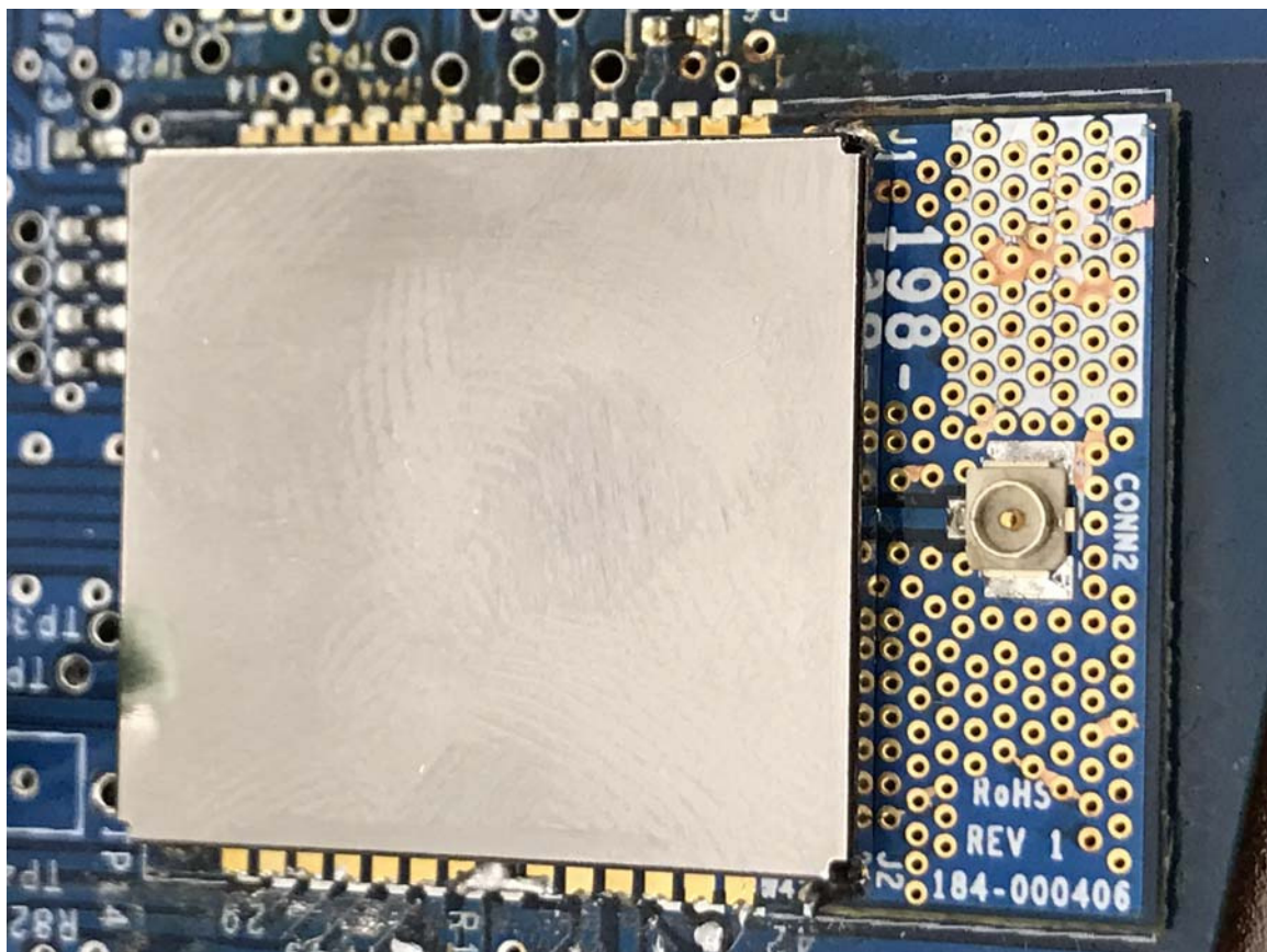
Front of module installed in host; Shield Installed (External Antenna)
