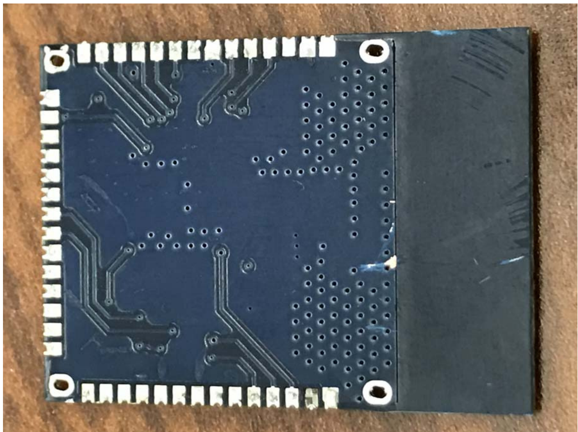
Rear of module (Chip Antenna)
