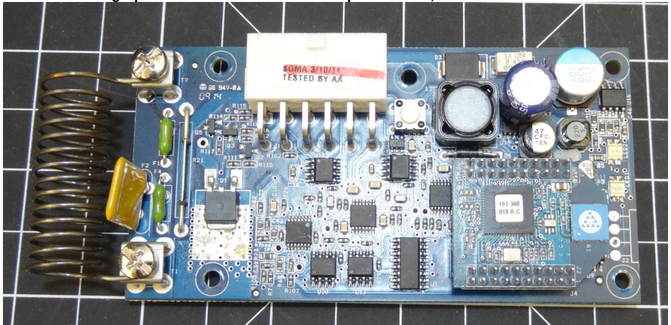
Photograph of Host Sensor Board: Component Side, Module shield removed
