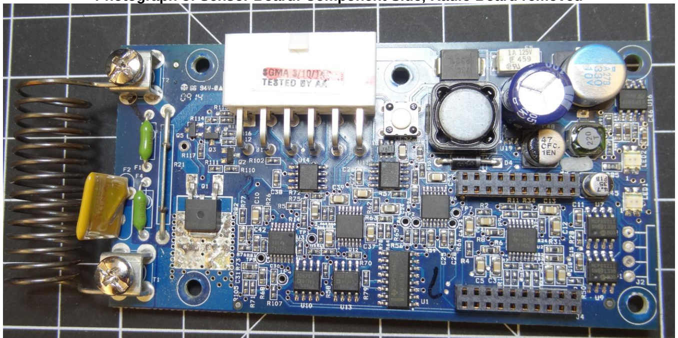
Photograph of Sensor Board: Component Side, Radio Board removed
