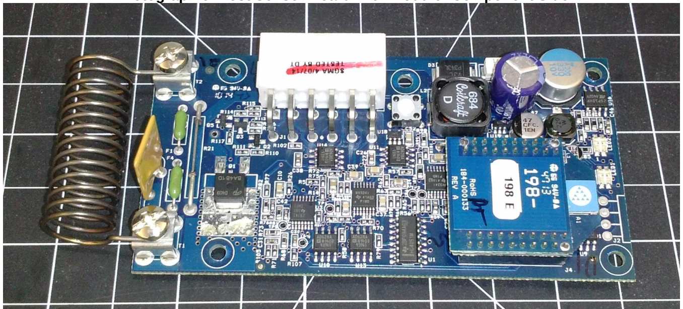
Photograph of host Sensor Board with Module: Component Side
