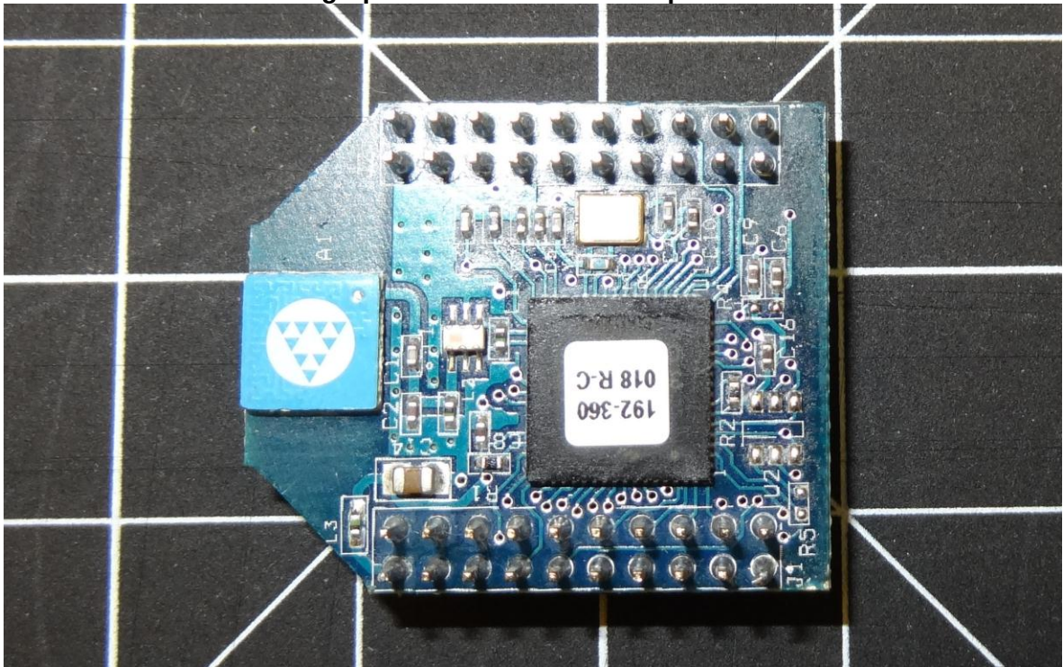
Photograph of Radio Board: Component Side
