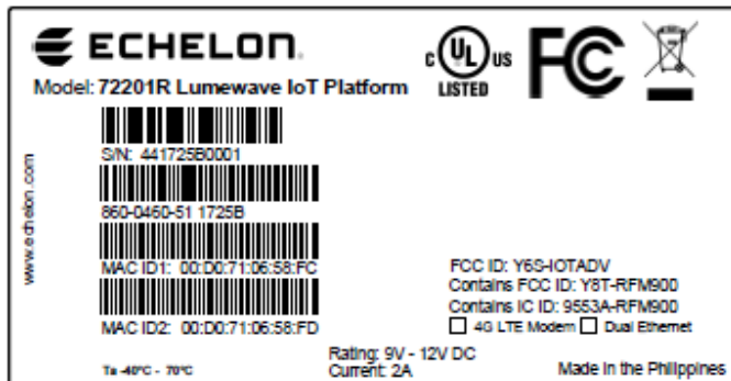
Product Label
