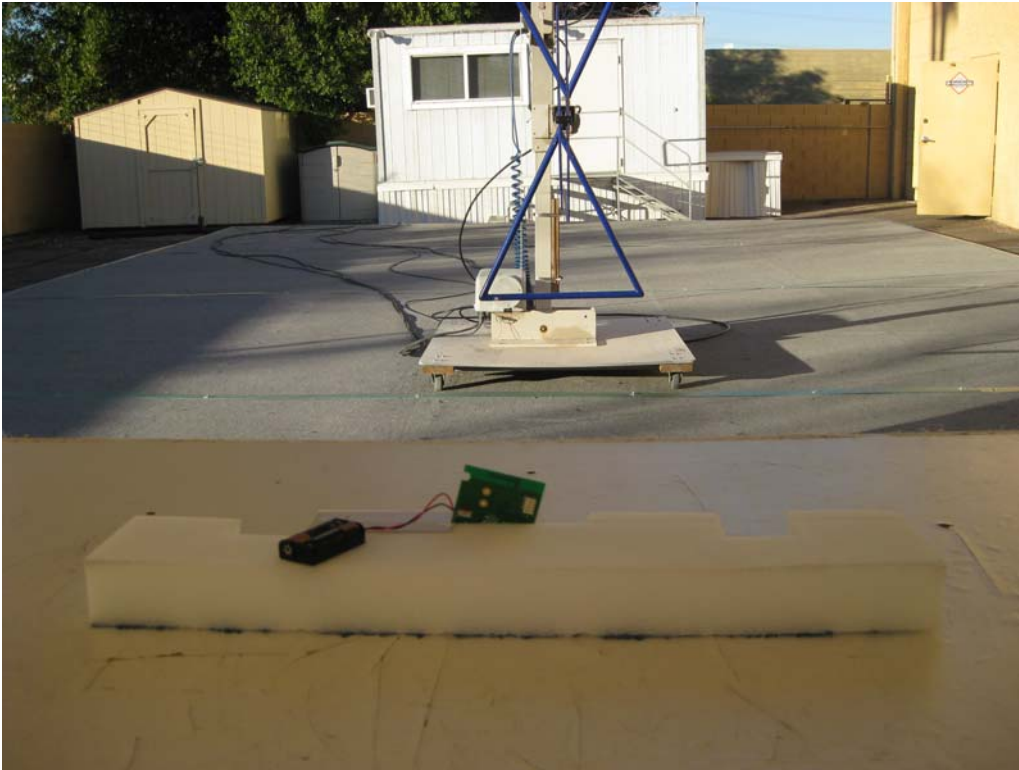
Radiated Emissions 30MHz – 1GHz #2
