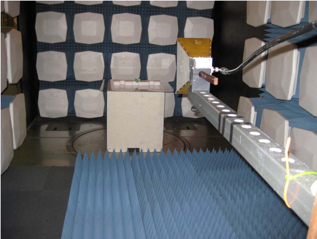
Radiated Tests above 1 GHz #2
