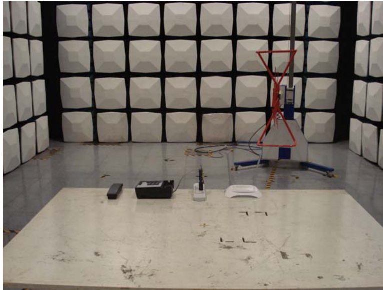
Radiated Emission Test Setup Front View
