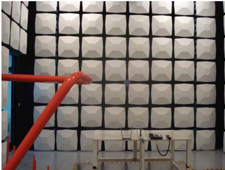
Radiated Emission Test Setup Rear View
