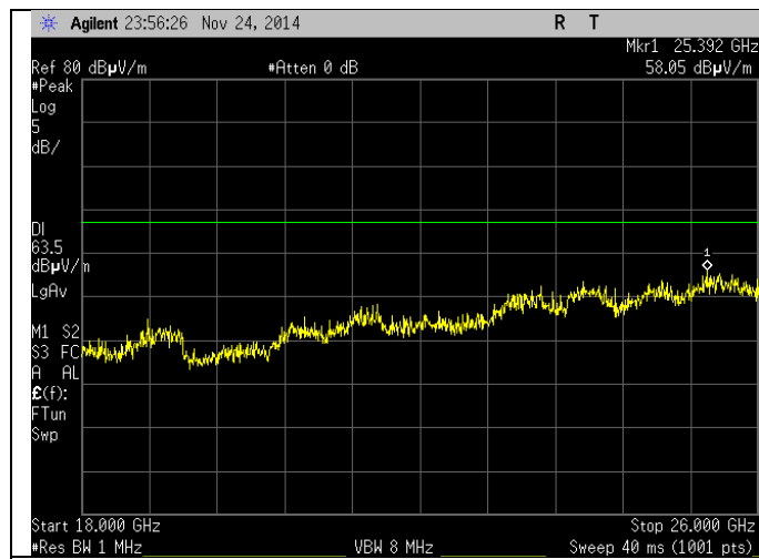
18-26 GHz Peak
