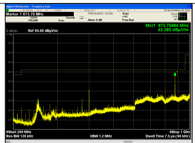
200-1000 MHz Horizontal
