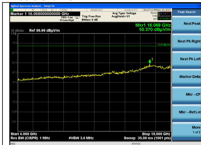
4-18 GHz Peak
