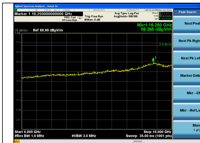
4-18 GHz (peak)
