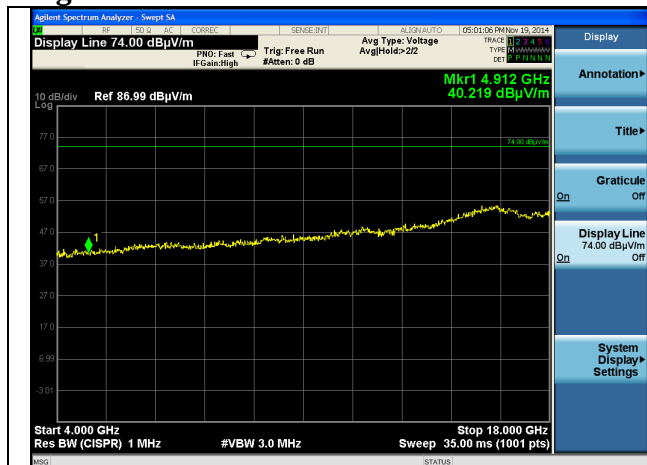
4-18 GHz Peak
