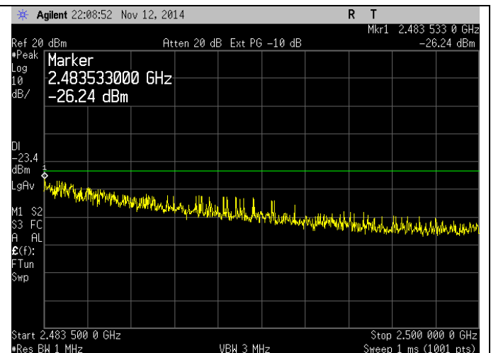
Peak
