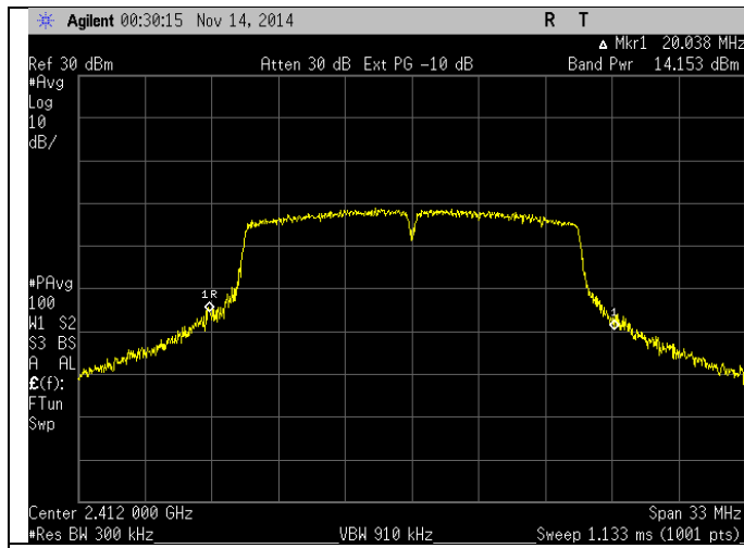
Output Power
