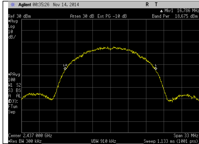
Output Power
