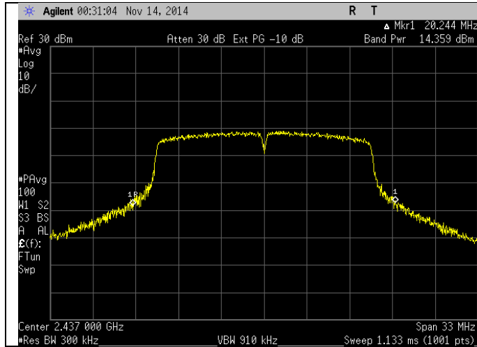
Output Power
