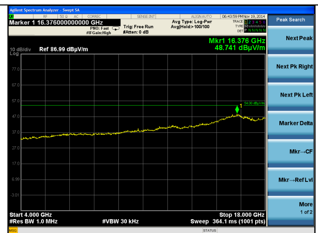
4-18 GHz (reduced VBW)
