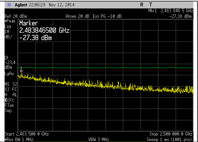
Peak
