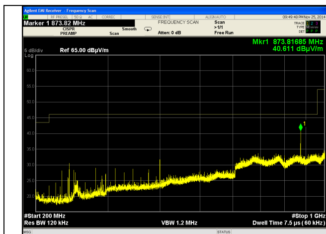
200-1000 MHz Vertical
