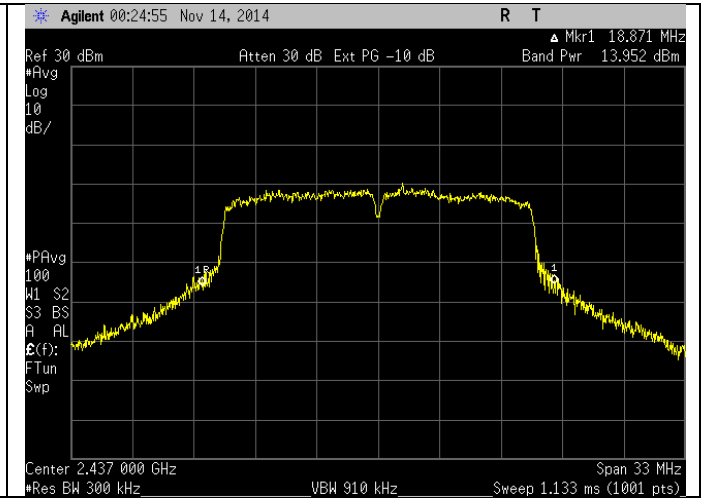
Output Power (24 Mbps)
