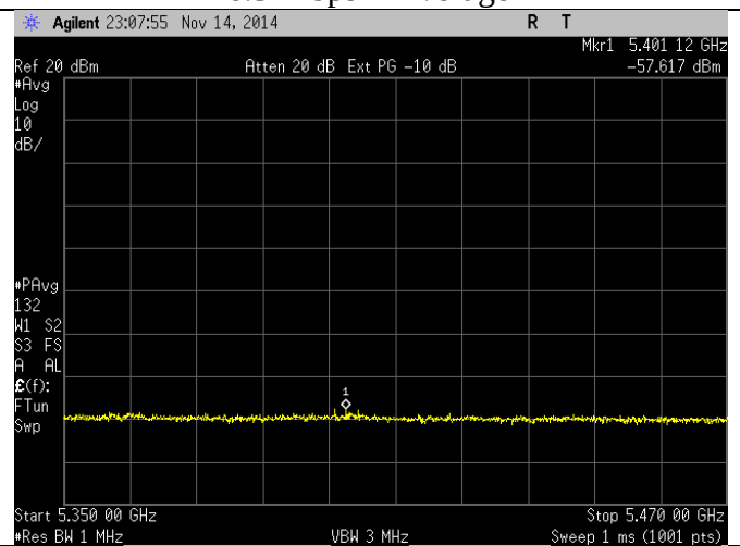
65 Mbps – Average
