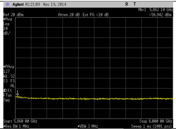
54 Mbps – Average
