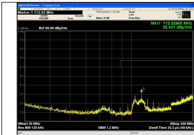
30-200 MHz Vertical
