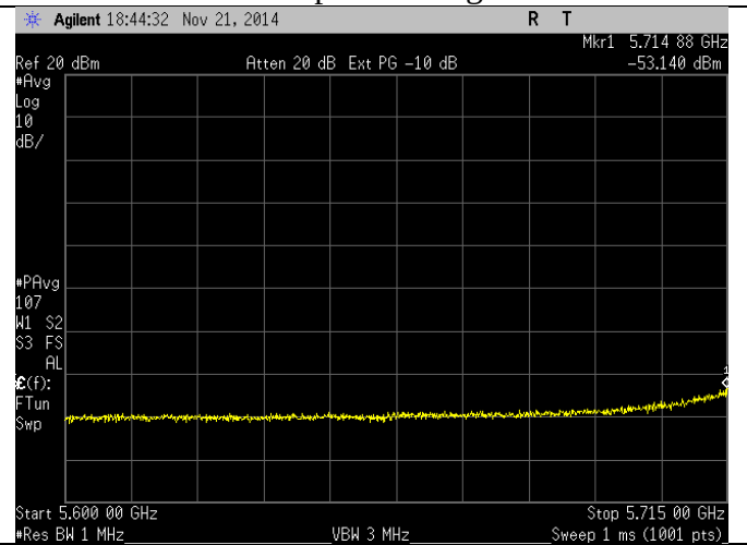
12 Mbps – Average
