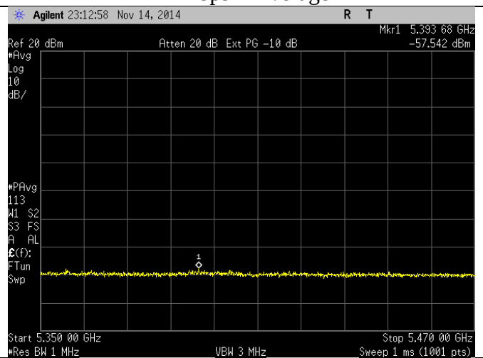
24 Mbps – Average
