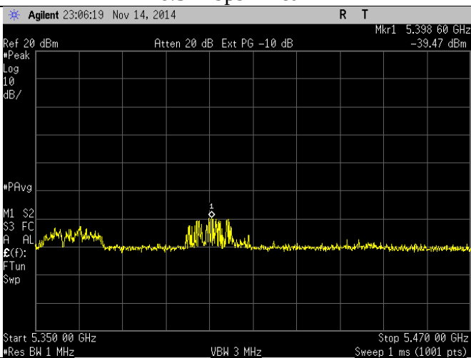
65 Mbps – Peak
