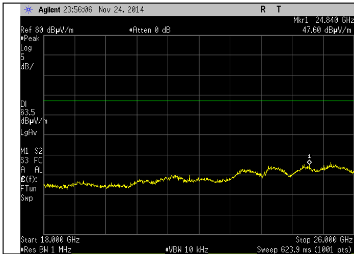
18-26 GHz – Average
