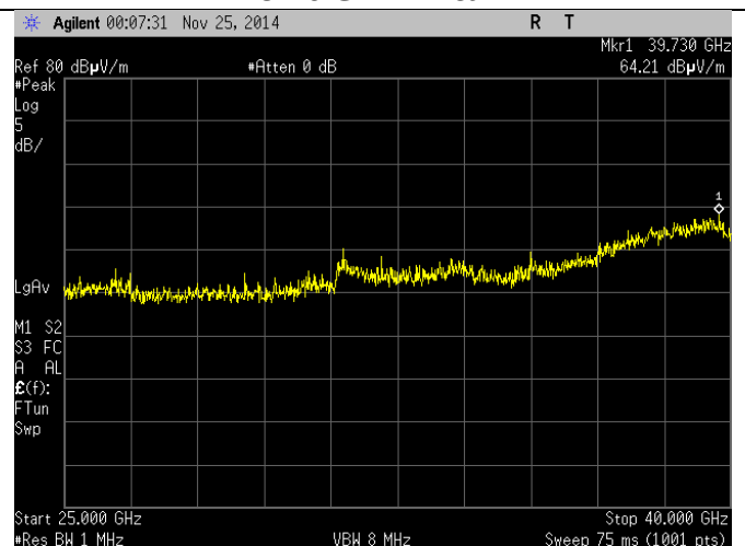
25-40 GHz – Peak
