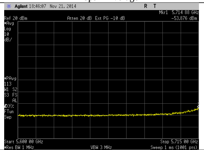
24 Mbps – Average
