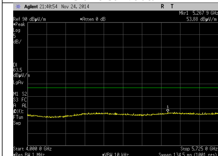
Channel 149 - Vertical
