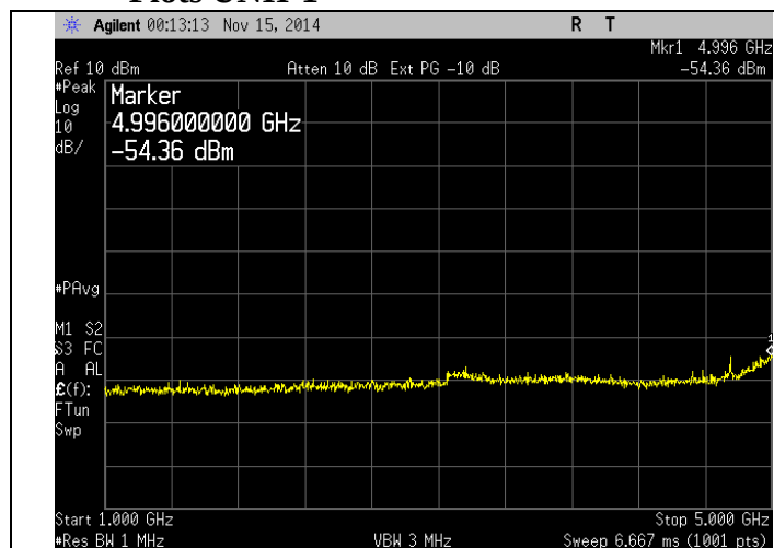
Low Channel - 1-5 GHz
