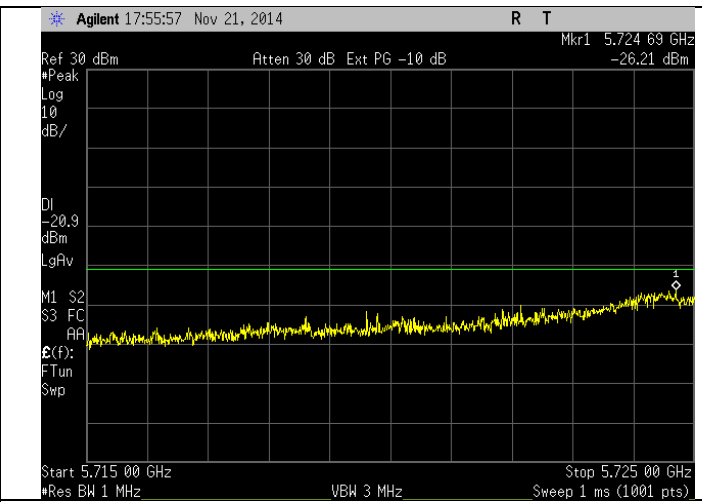
12 Mbps – Peak
