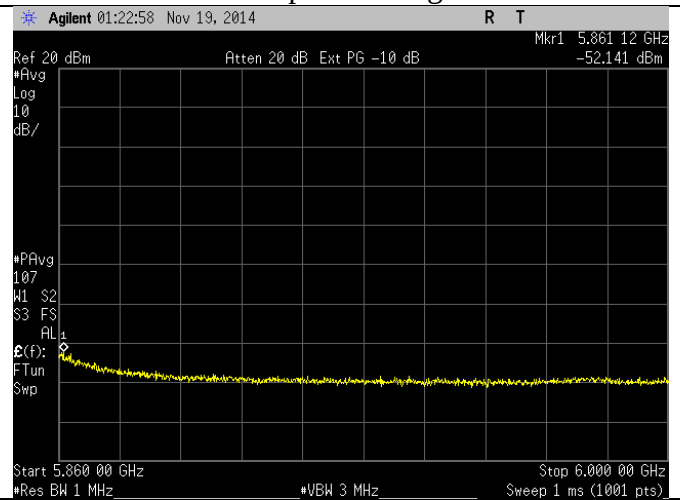
12 Mbps – Average
