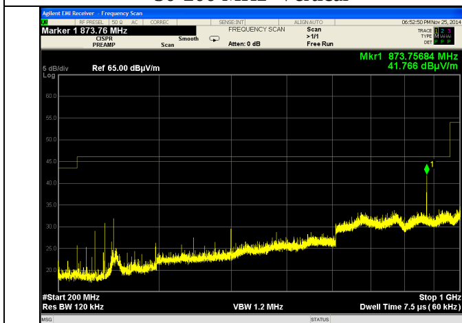
200-1000 MHz Vertical
