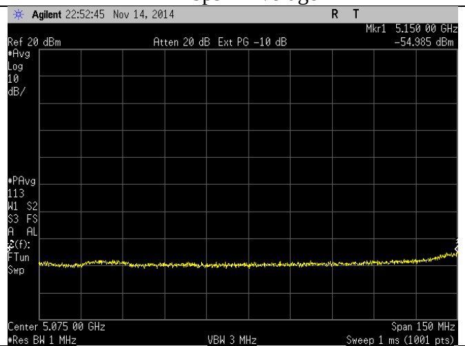
24 Mbps – Average
