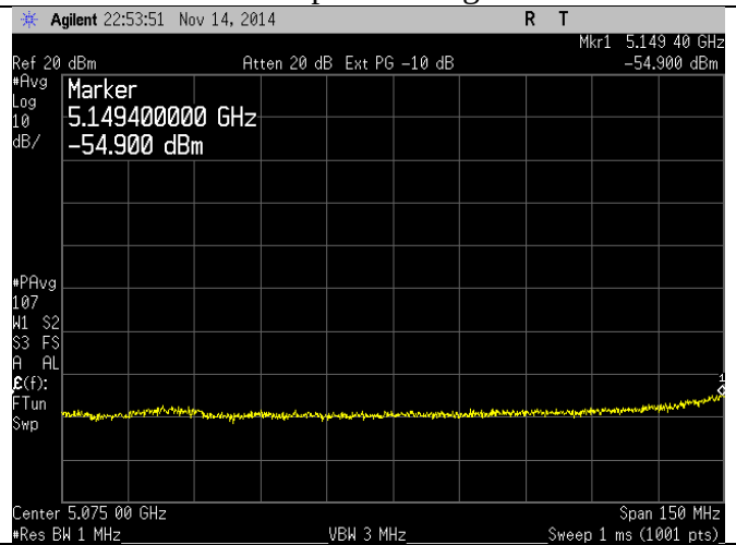
12 Mbps – Average
