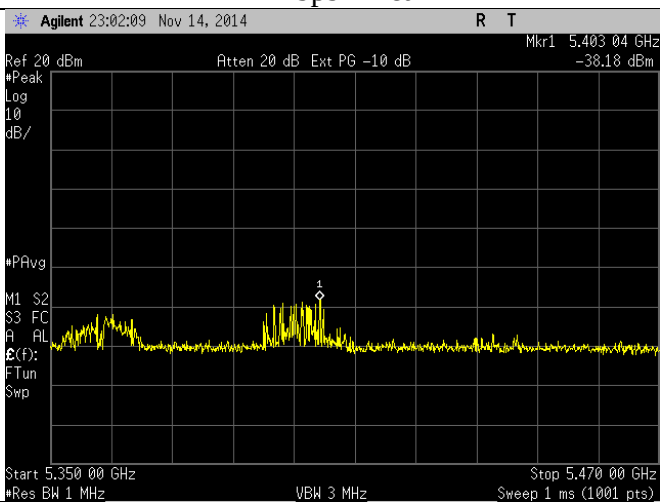
24 Mbps – Peak
