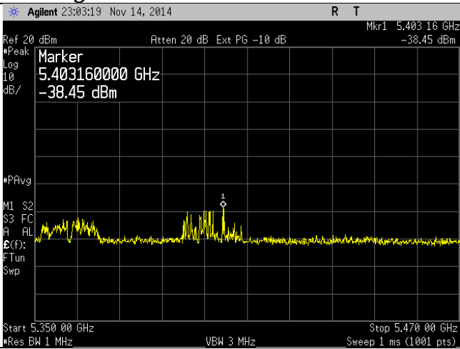
54 Mbps – Peak
