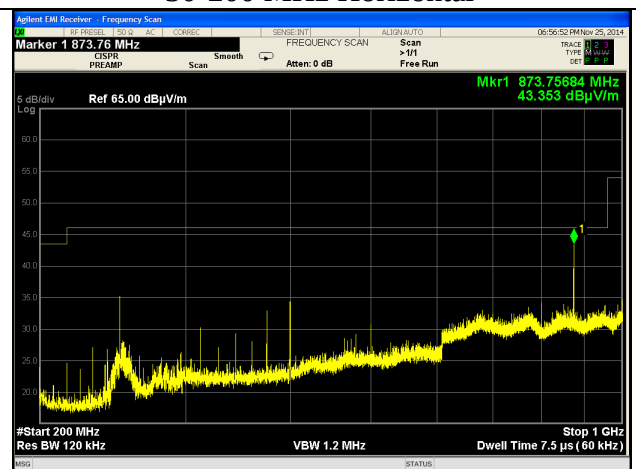
200-1000 MHz Horizontal
