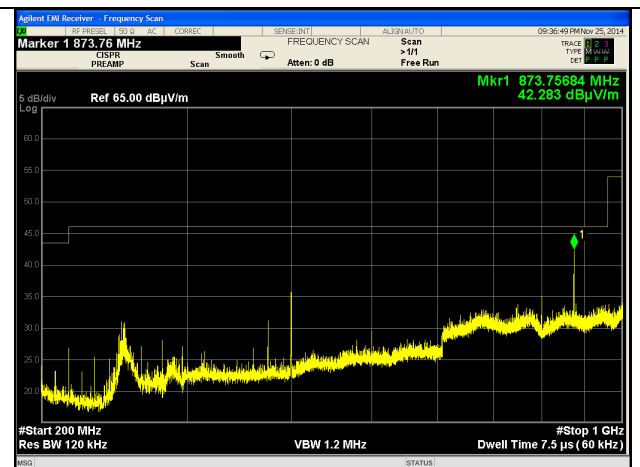
200-1000 MHz Horizontal
