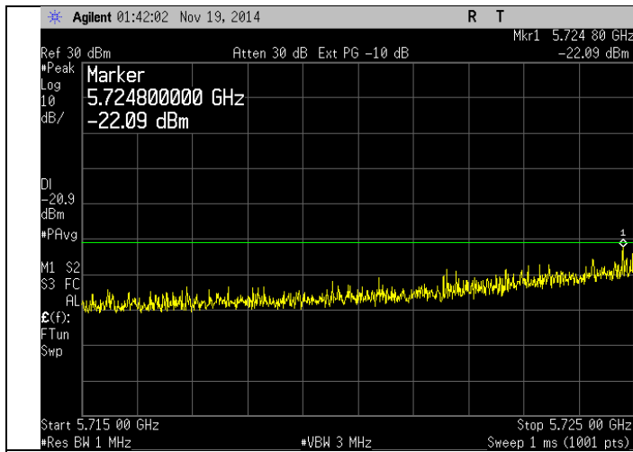
6 Mbps – Peak
