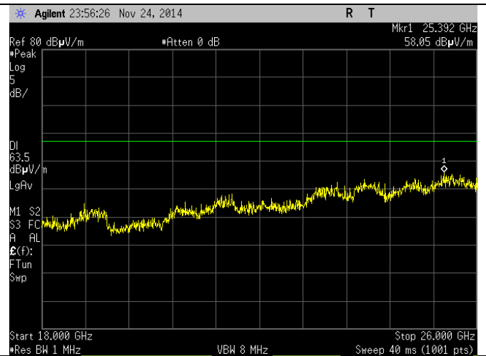
18-26 GHz – Peak
