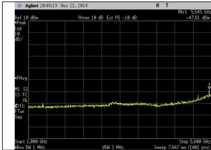
Low Channel - 1-5.6 GHz
