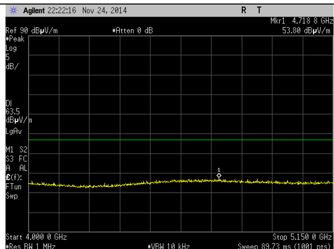
Channel 36 - Horizontal
