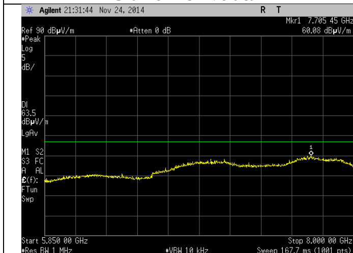
Channel 165 - Vertical
