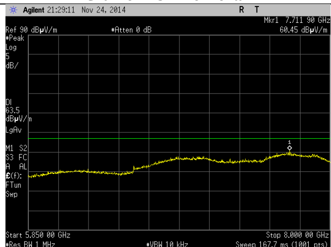
Channel 165 - Horizontal
