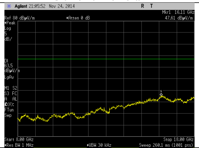
Channel 157 - Horizontal
