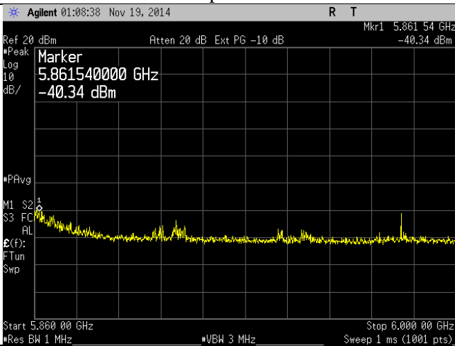
12 Mbps – Peak
