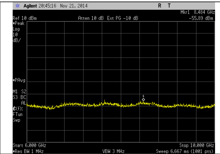
Low Channel - 6-10 GHz
