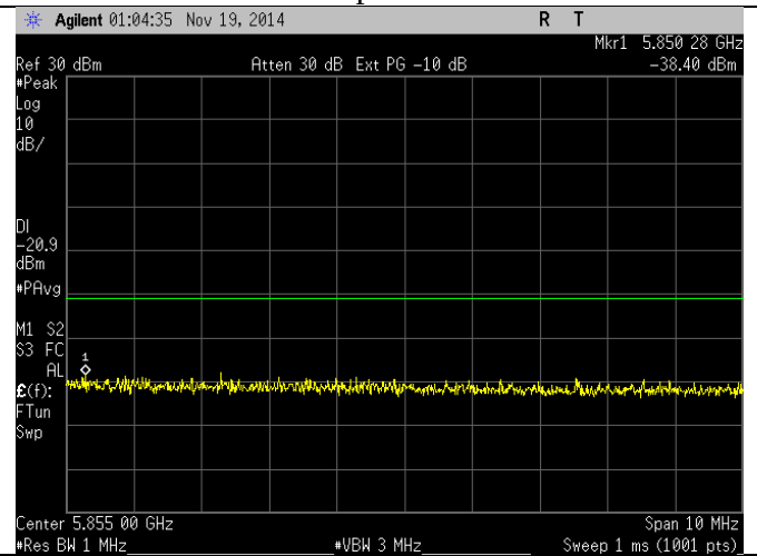
54 Mbps – Peak
