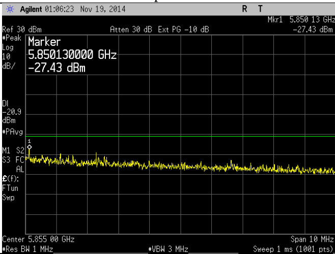
24 Mbps – Peak
