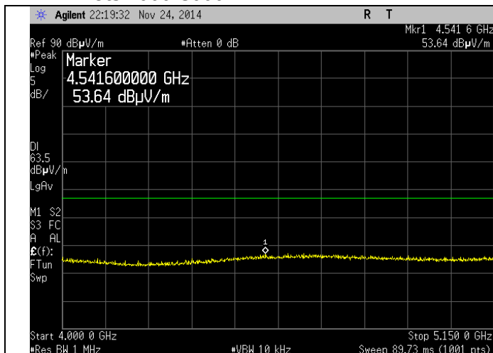
Channel 36 - Vertical
