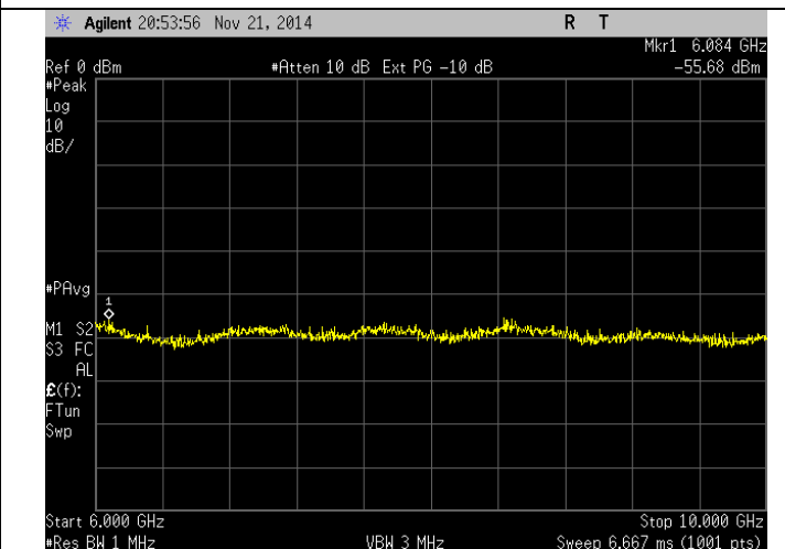
High Channel - 6-10 GHz
