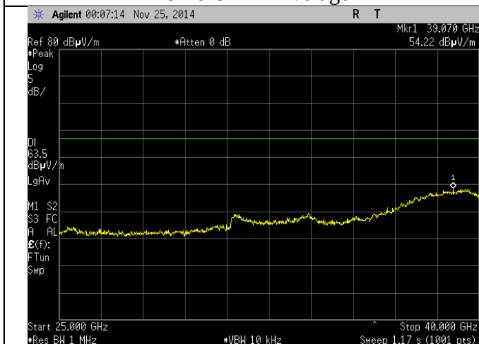
25-40 GHz – Average
