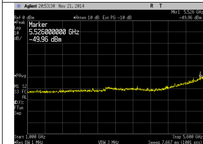
High Channel - 1-5.6 GHz
