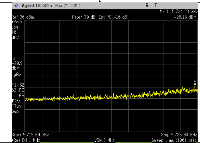
54 Mbps – Peak
