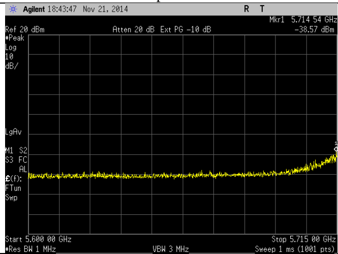
12 Mbps – Peak
