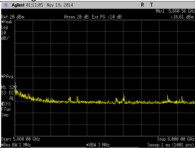
6 Mbps – Peak
