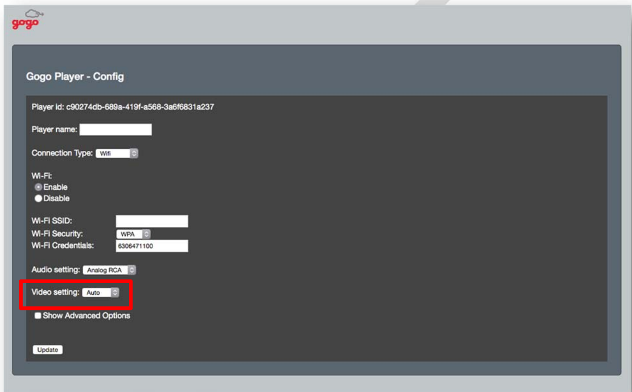
Figure 4.10. Video Setting
