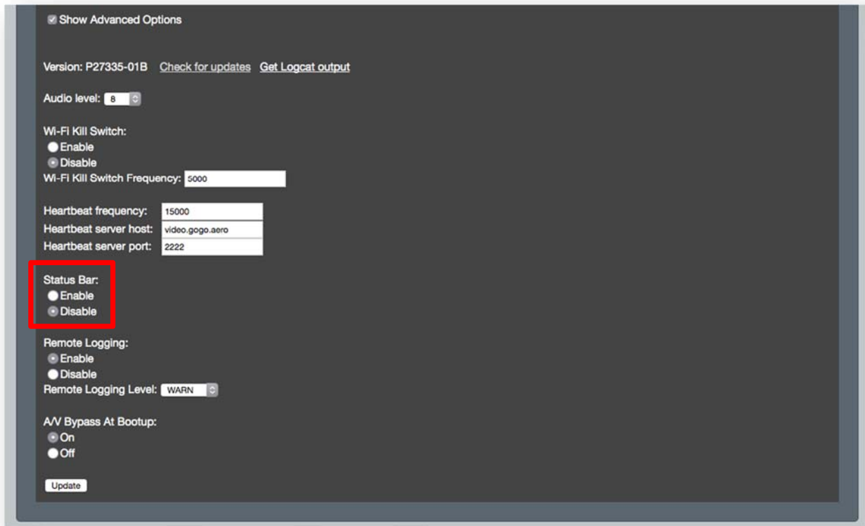
Figure 4.17. Status Bar
