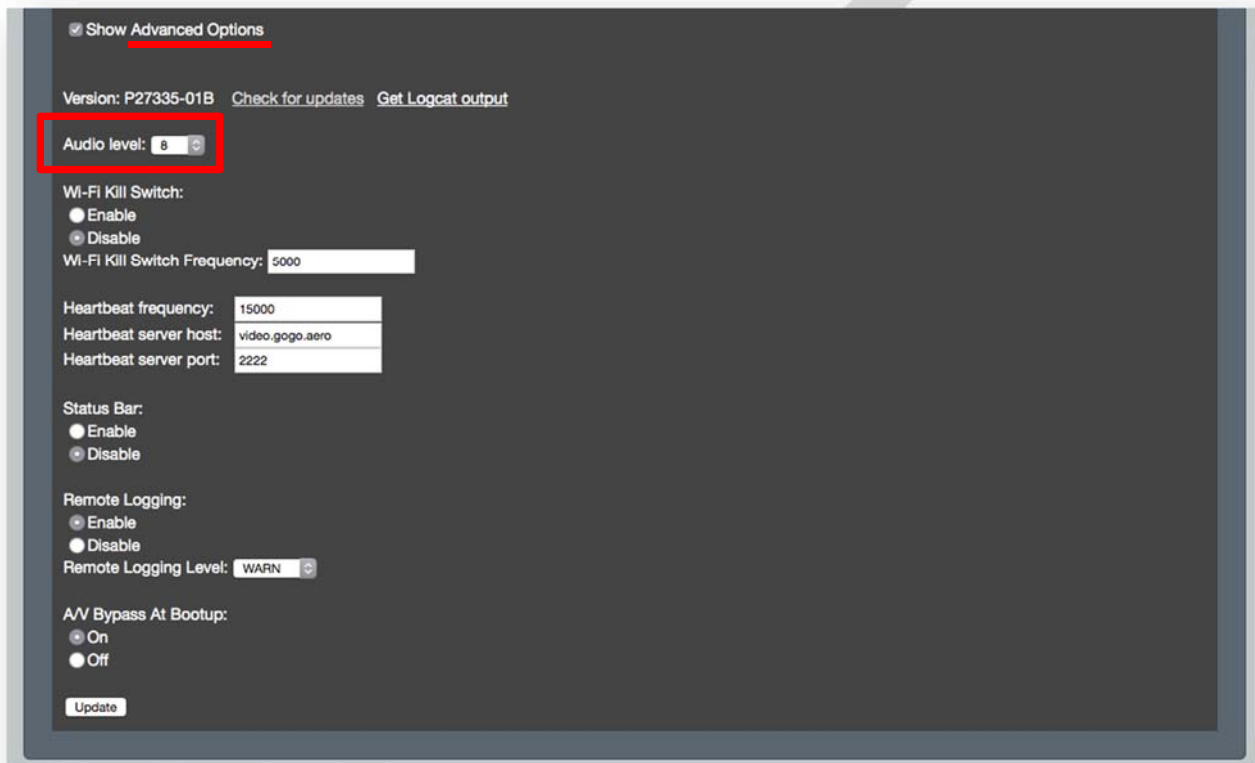
Figure 4.13. Audio Level
