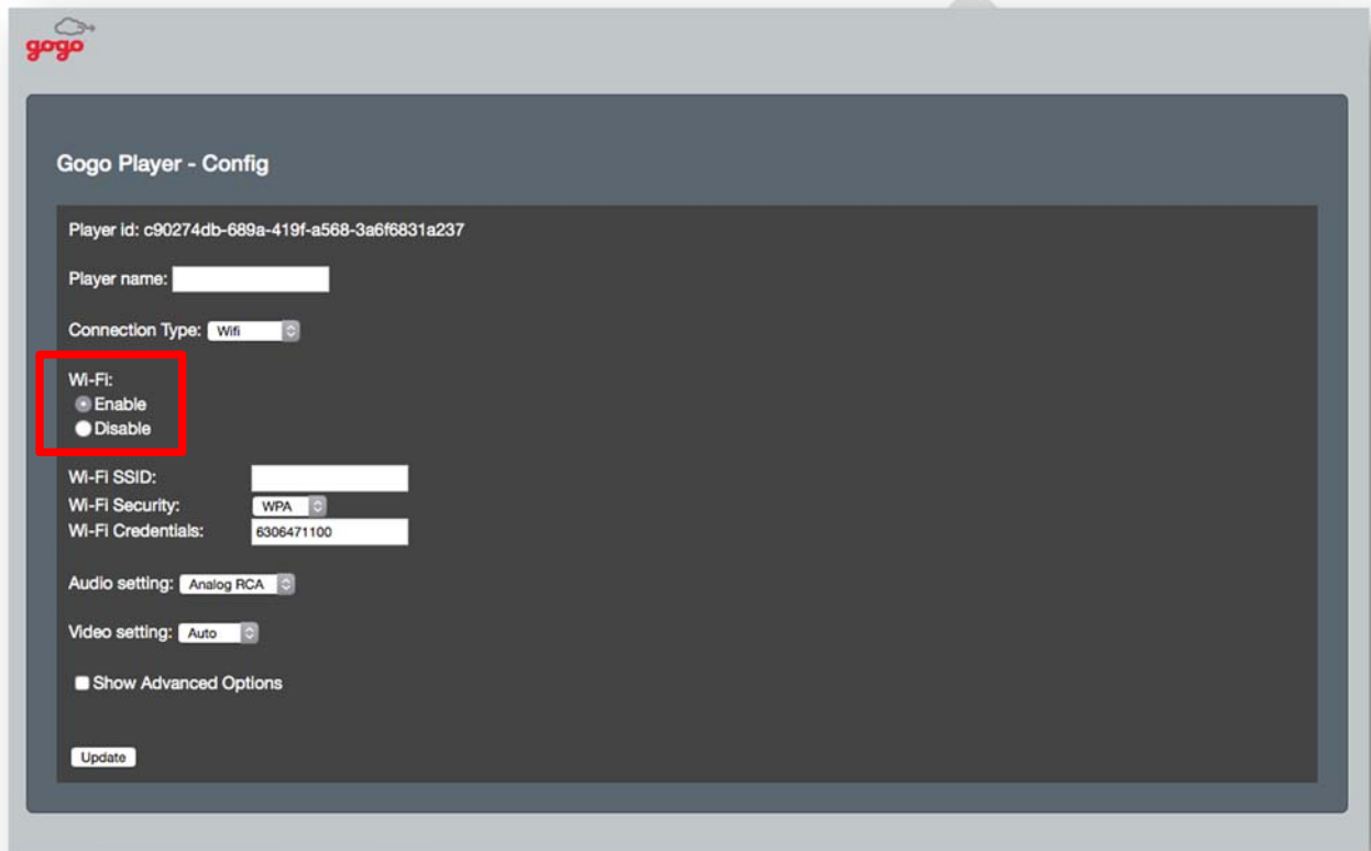
Figure 4.7. Wi-Fi: Enable/Disable
