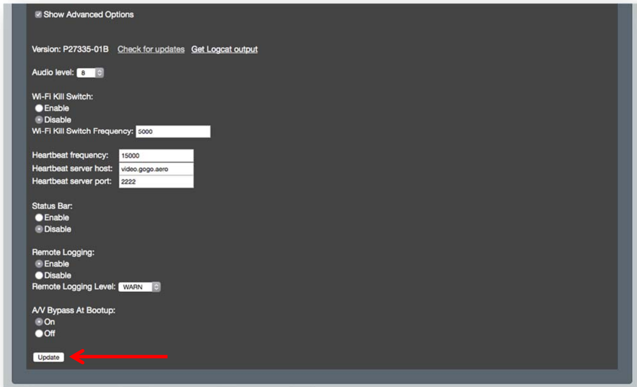
Figure 4.21. Update
