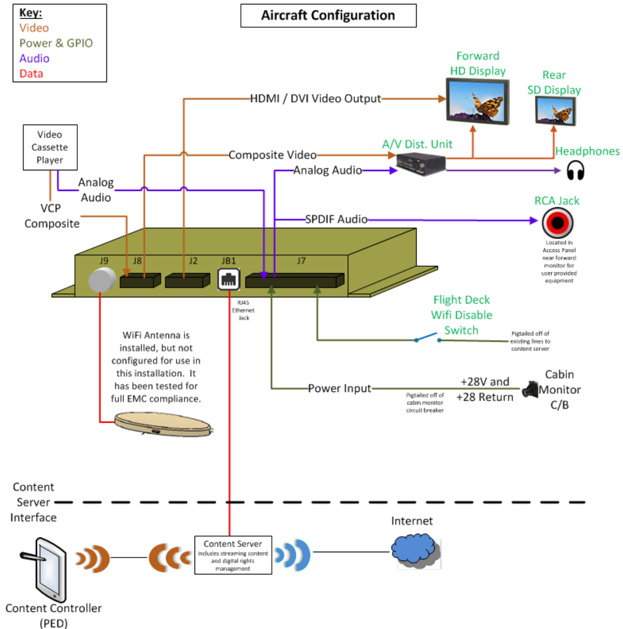
Figure 2.2. Sample GVPV Installation
