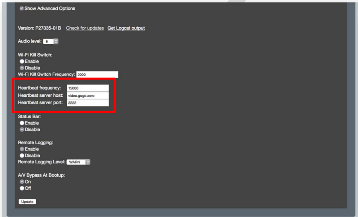
Figure 4.16. Heartbeat Frequency/Host/Port
