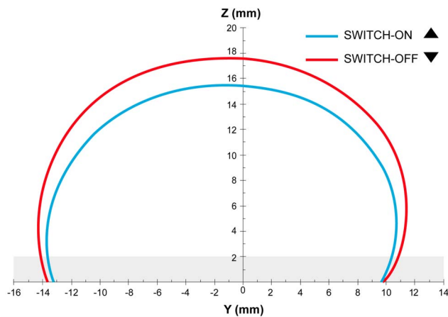
Typical switch-on and switch-off sensing distances along Y axis as function of Z. (longitudinal misalignment for X=0 )
