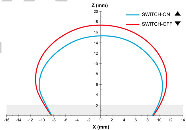
Typical switch-on and switch-off sensing distances along X axis as function of Z. (transverse misalignment for Y=0 )
