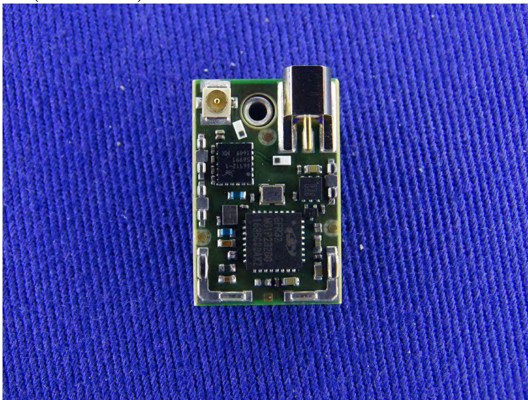
(19) EUT Photo (M/N: EMIP400s)
