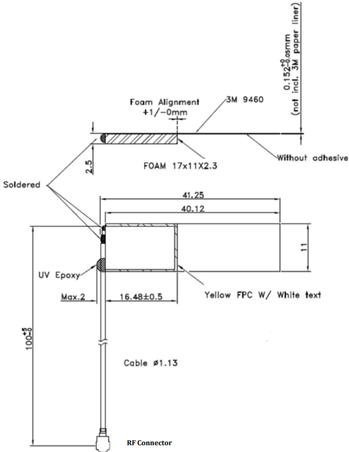
Figure 3: FlexPIFA mechanical drawing of 001-0025
