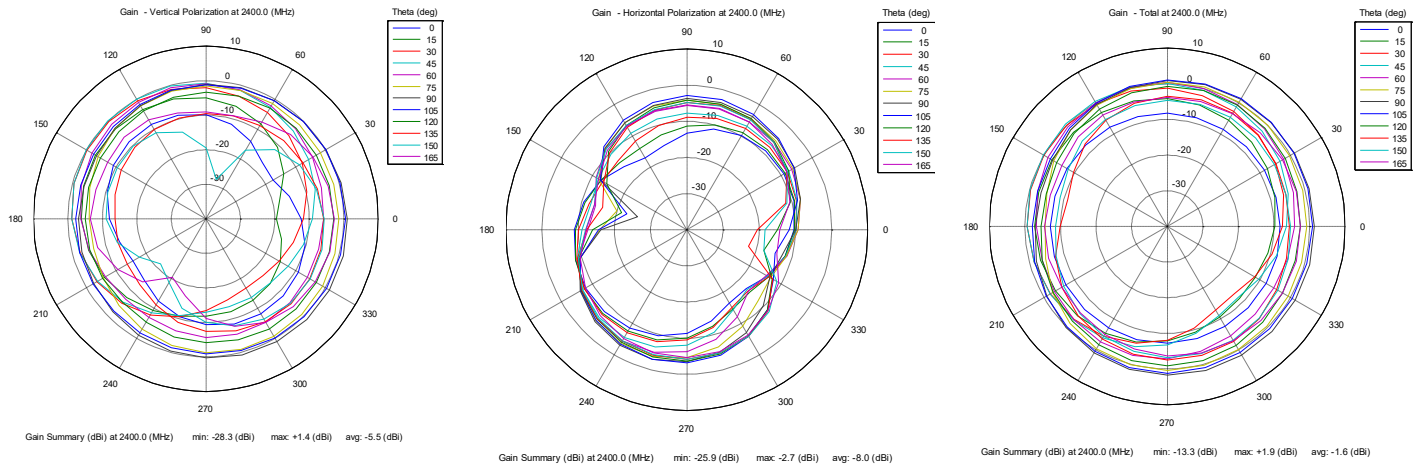
Figure 7: Vertical, horizontal, and total gain patterns – 2400 MHz
