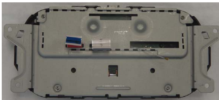
Figure10: VP2Refresh front unit back side view
