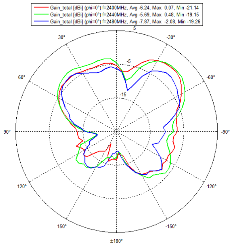
Figure4: measured X-Z plane, Z arrow =0°
