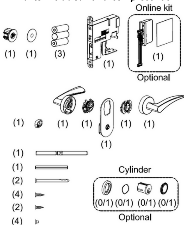
Figure 18: Parts included for a complete Essence lock; see details in Table 6 (ANSI DA), Table 7 (ANSI DB) and Table 8 (EURO). The online kit and cylinder kit are purchased separately, when applicable.
