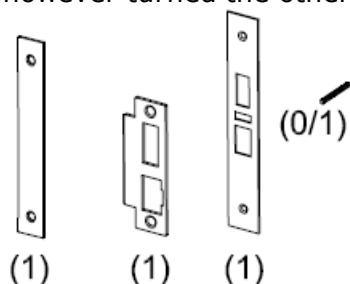
Figure 19, from the left: front for Essence cassette, striker plate ANSI, lock front ANSI and cylinder set screw for cylinders ex threaded ANSI ADB.
