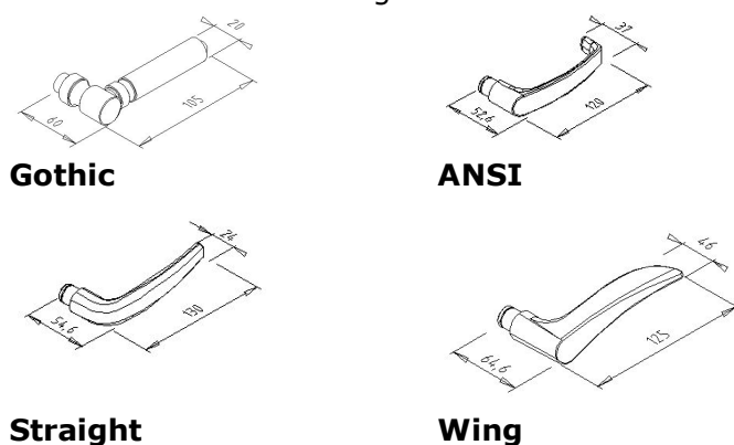
Figure 13: Standard Essence door handles
