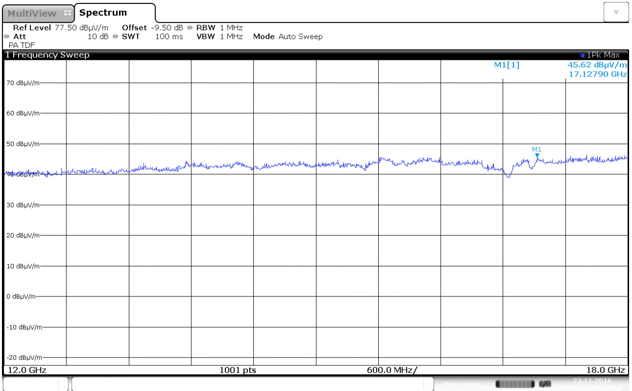
Radiated Emissions ch. 2404 MHz, 12 – 18 GHz, VP, @1m – Pre-scan
