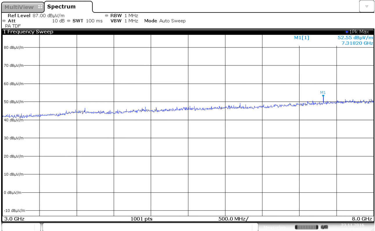
Radiated Emissions ch. 2440 MHz, 3 – 8 GHz, VP, @3m – Pre-scan
