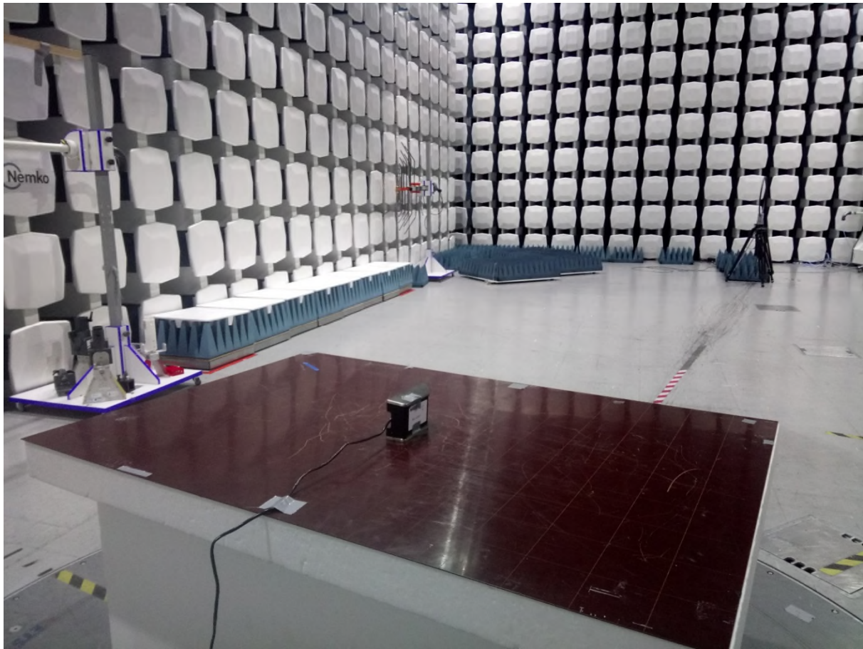
Below 30MHz
