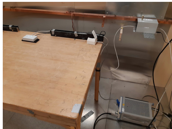
Power-Line Conducted Emissions
