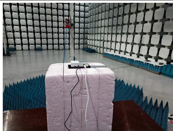
Radiated Emissions 1 – 18 GHz
