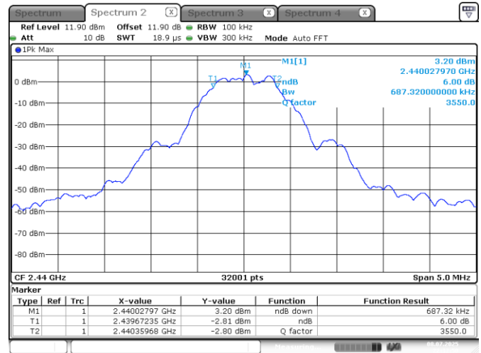
Figure 7.5-2: 6 dB bandwidth on Mid Channel plot
