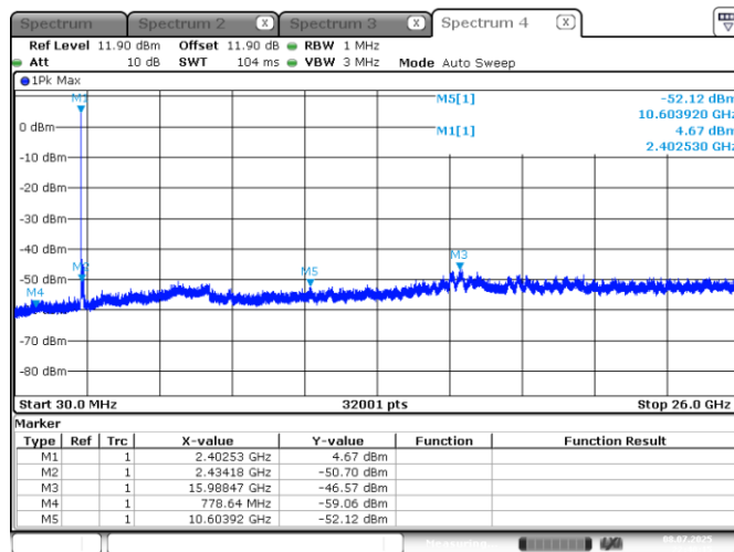
Figure 7.7-3: Conducted spurious emissions on Low Channel
