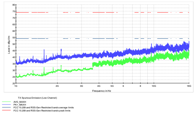
Figure 7.7-61: Radiated spurious emissions on Low Channel (1-18 GHz)
