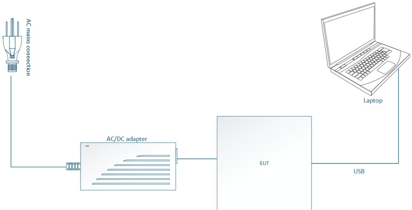
Figure 4.5-1: Radiated testing block diagram
