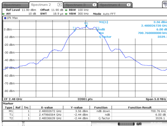
Figure 7.5-3: 6 dB bandwidth on High Channel plot
