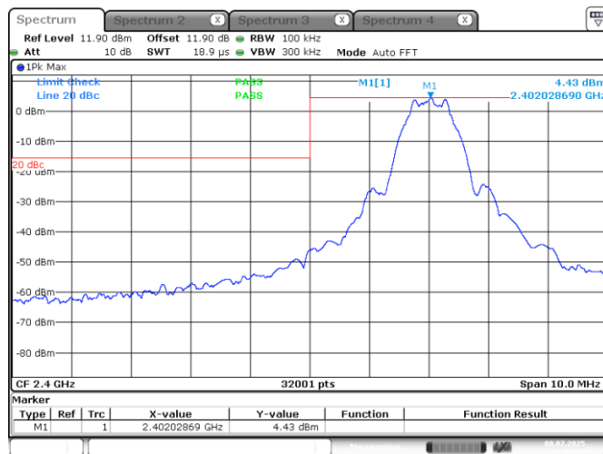
Figure 7.7-1: Band edge conducted spurious emissions at 2400 MHz
