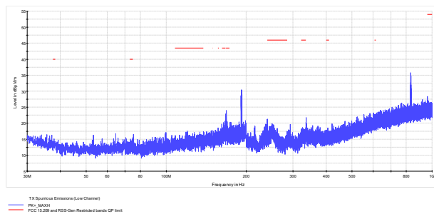
Figure 7.7-8: Radiated spurious emissions on Low Channel (<1 GHz)
