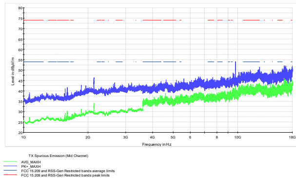
Figure 7.7-12: Radiated spurious emissions on Mid Channel (1-18 GHz)
