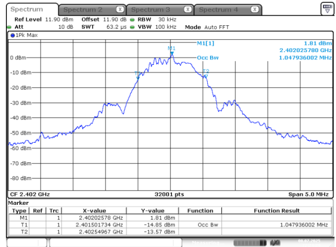
Figure 7.5-4: 99% occupied bandwidth on Low Channel plot
