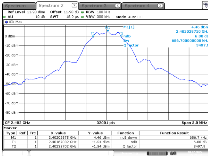
Figure 7.5-1: 6 dB bandwidth on Low Channel plot
