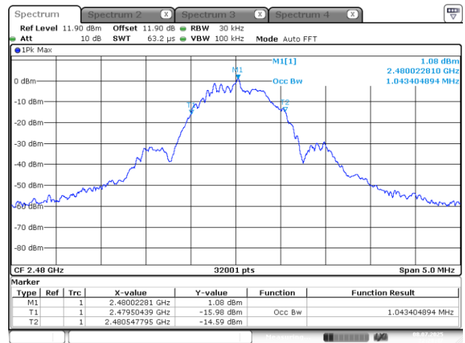
Figure 7.5-6: 99% occupied bandwidth on High Channel plot
