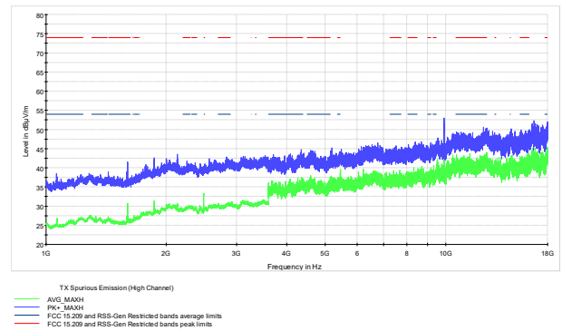
Figure 7.7-13: Radiated spurious emissions on High Channel (1-18 GHz)
