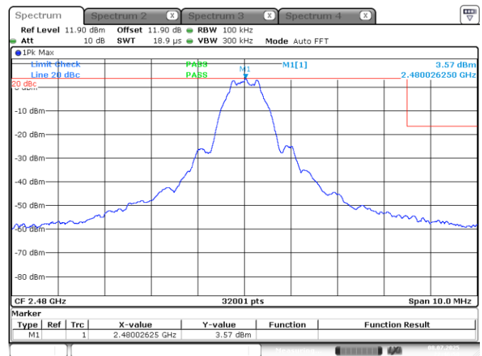
Figure 7.7-2: Band edge conducted spurious emissions at 2483.5 MHz
