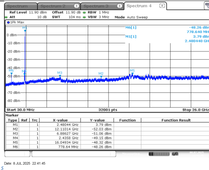
Figure 7.7-5: Conducted spurious emissions on High Channel
