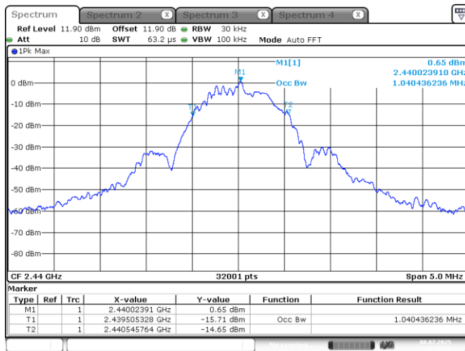
Figure 7.5-5: 99% occupied bandwidth on Mid Channel plot
