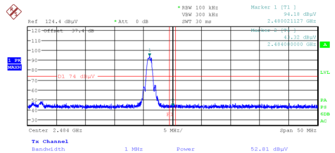
Figure 7.7-7: Radiated spurious emissions on upper band edge, 2483.5 MHz
