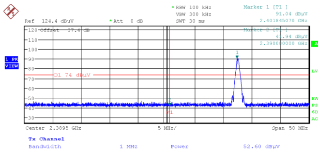
Figure 7.7-6: Radiated spurious emissions on lower band edge, 2390 MHz
