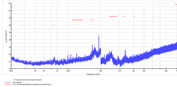
Figure 7.7-10: Radiated spurious emissions on High Channel (<1 GHz)
