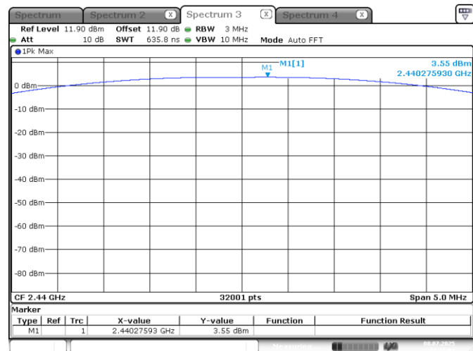
Figure 7.6-2: Output power on mid channel
