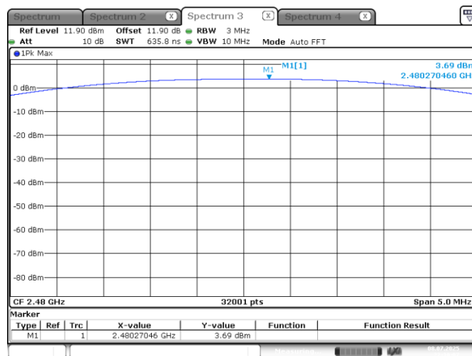
Figure 7.6-3: Output power on high channel
