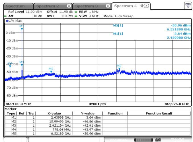
Figure 7.7-4: Conducted spurious emissions on Mid Channel
