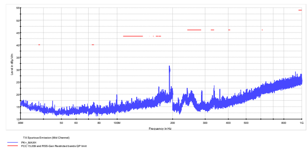
Figure 7.7-9: Radiated spurious emissions on Mid Channel (<1 GHz)
