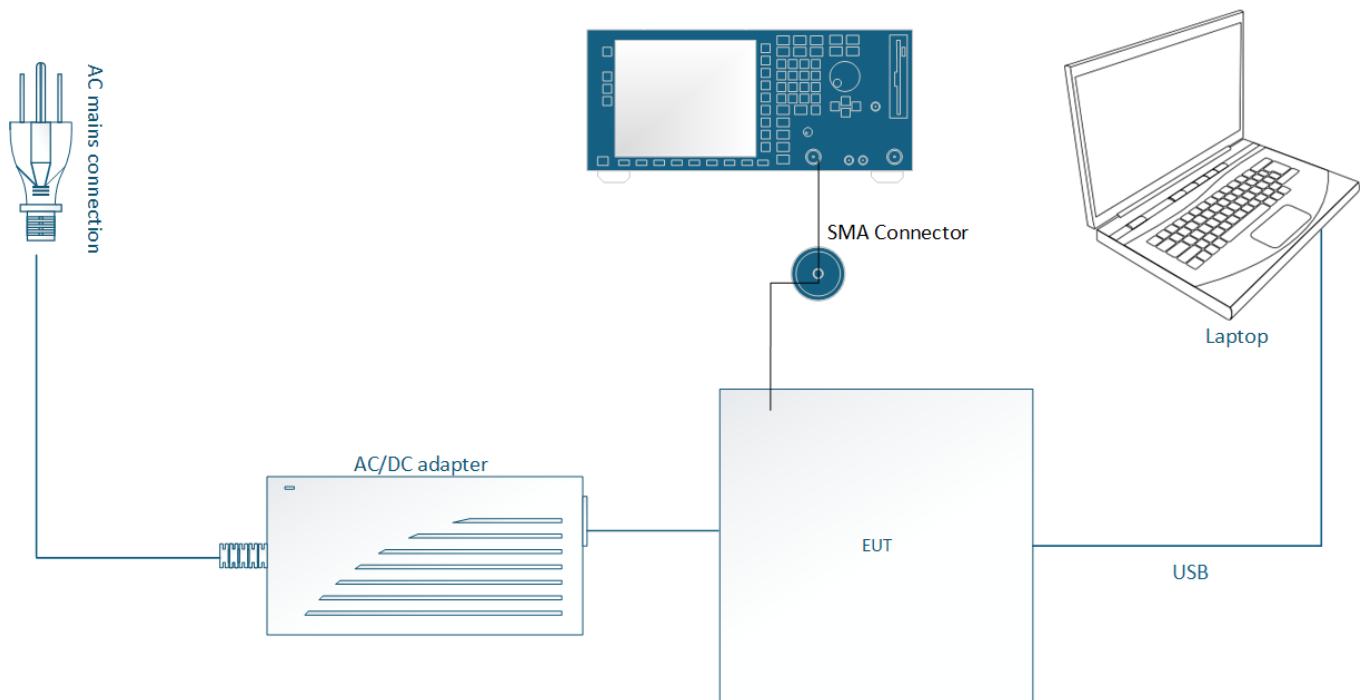
Figure 4.5-2: Antenna port testing block diagram
