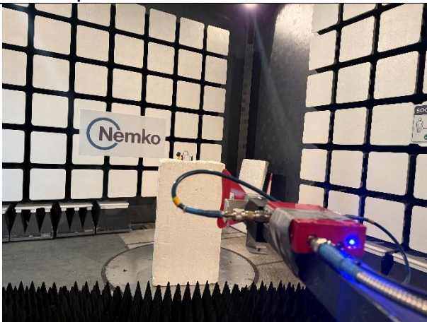
Radiated Spurious Emissions 1-18 GHz
