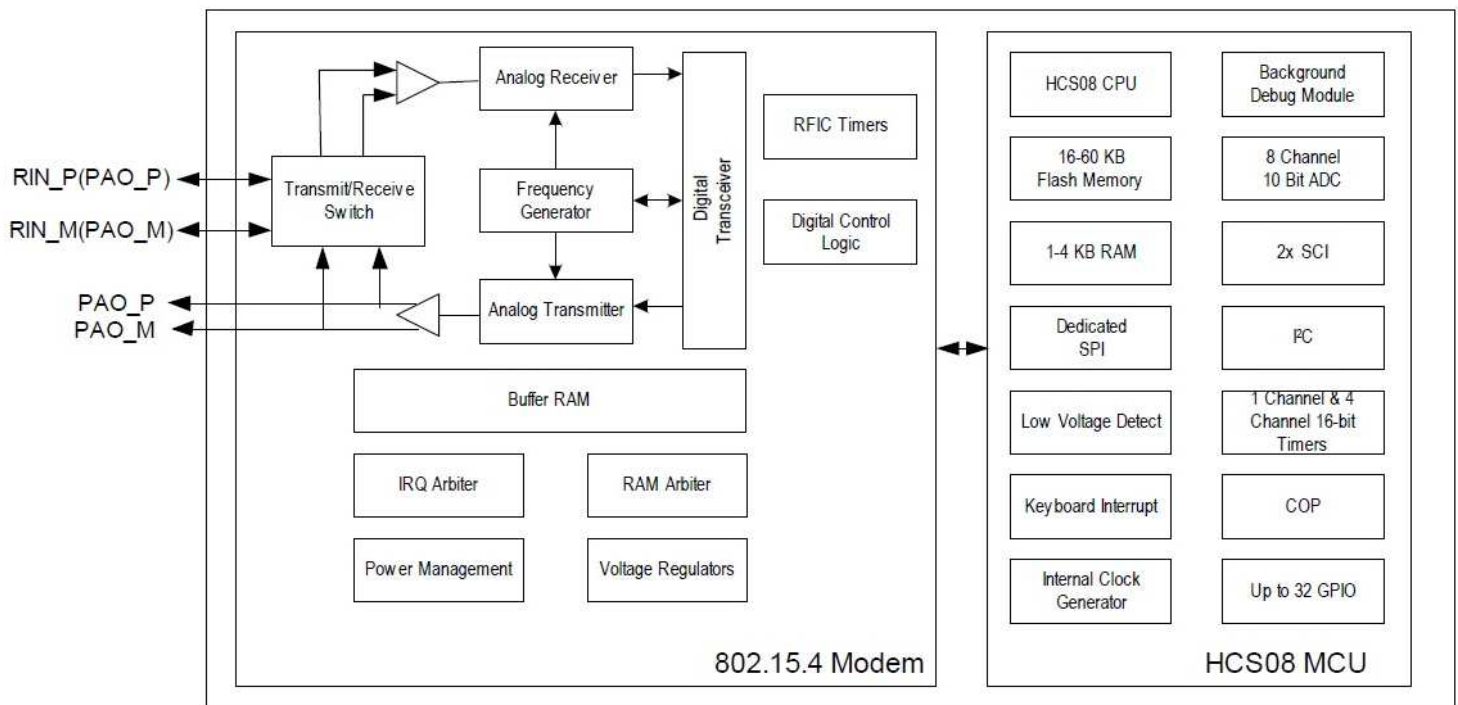
MC1321x System Level Block Diagram
