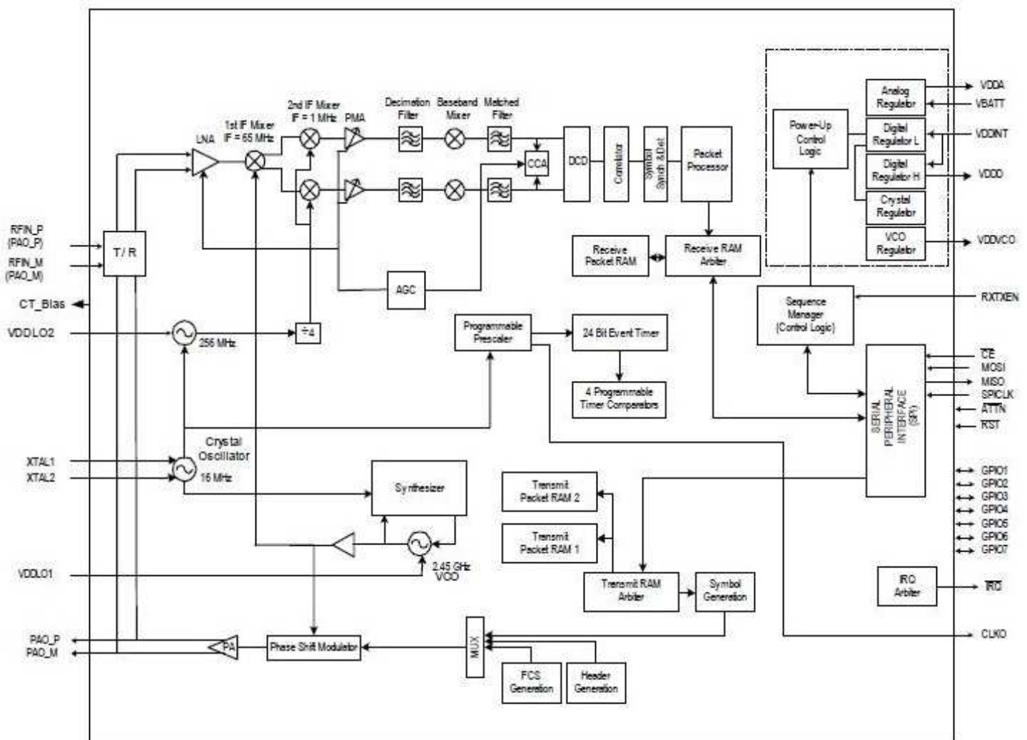
802.15.4 Modem Block Diagram
