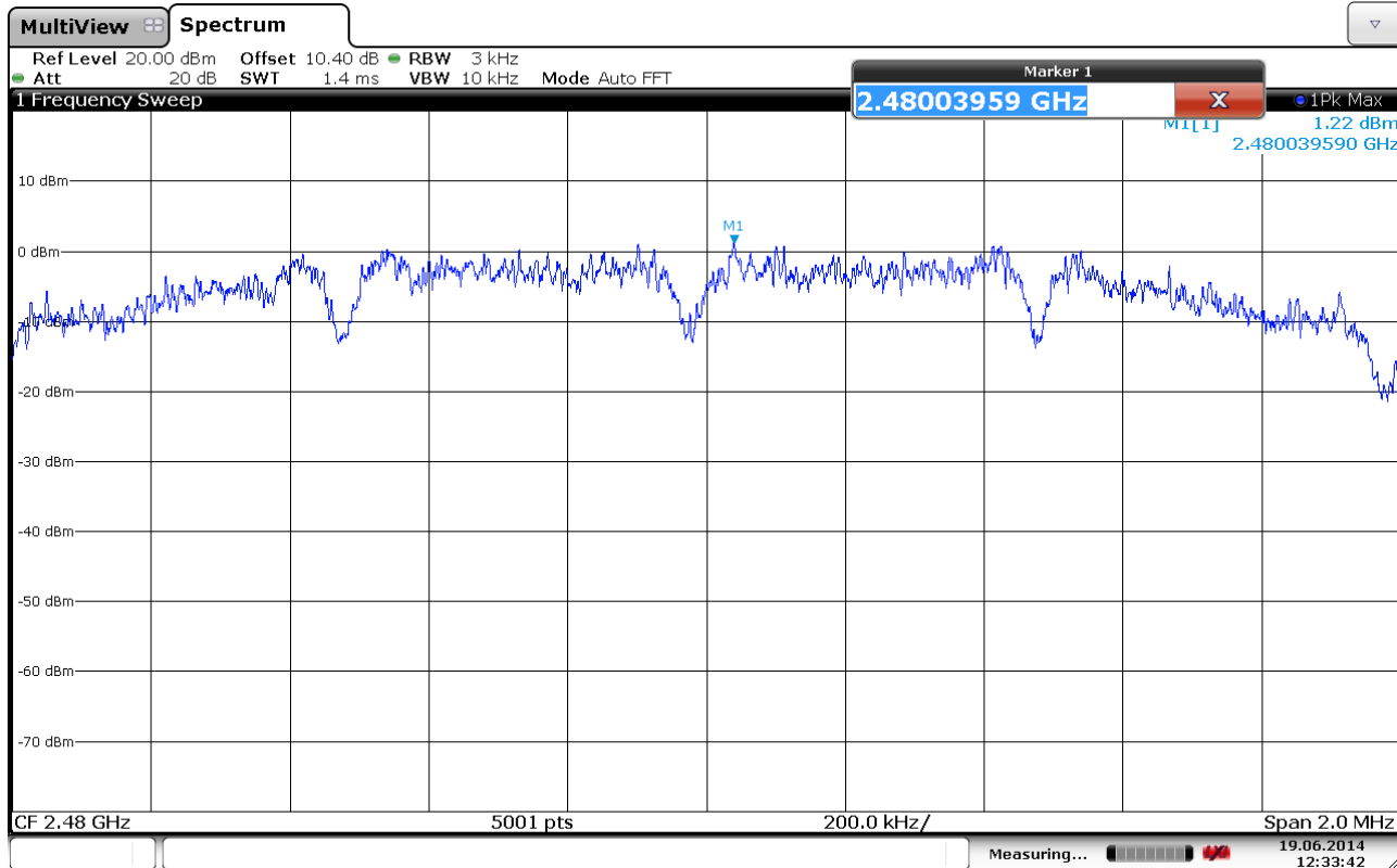
Conducted measurement, Ch 2480 MHz
