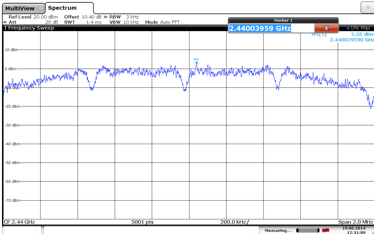
Conducted measurement, Ch 2440 MHz
