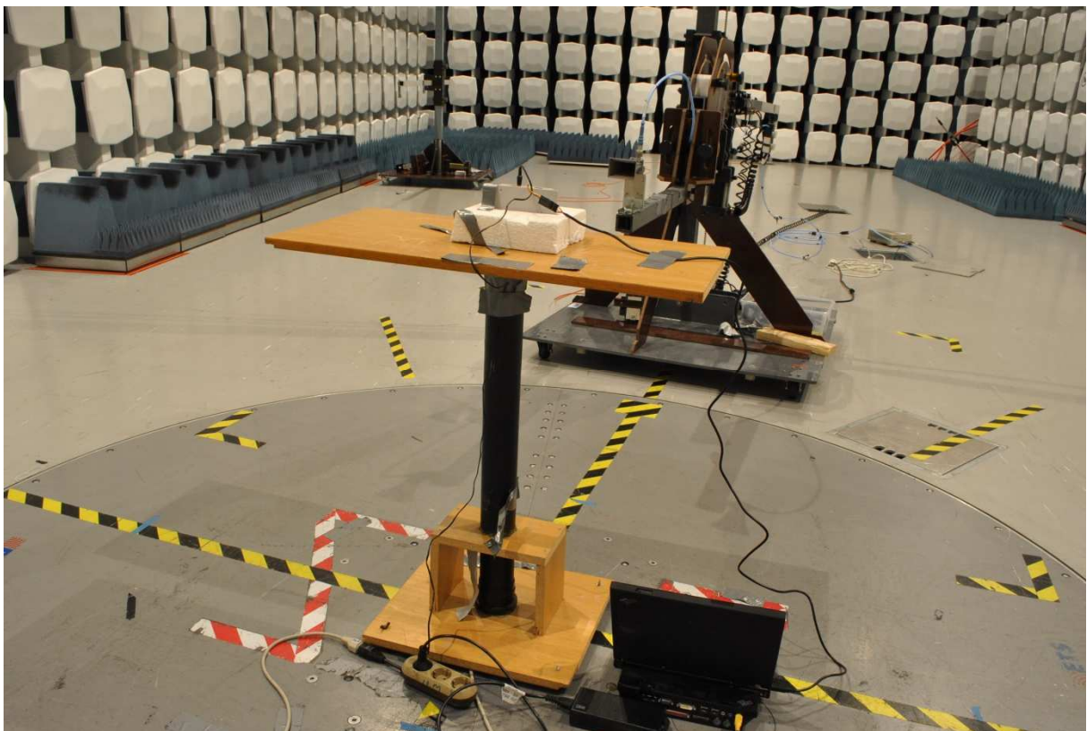
Radiated emissions 8.5 – 12 GHz
