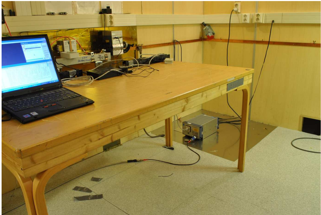
Power-Line Conducted emissions, Power over Ethernet
