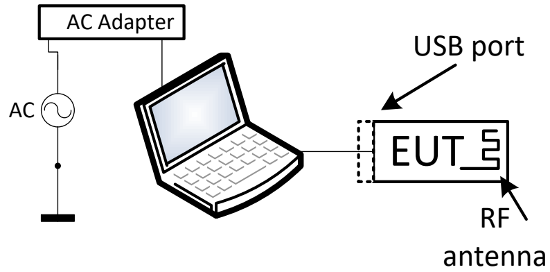
Figure 3.6-1: Setup diagram
