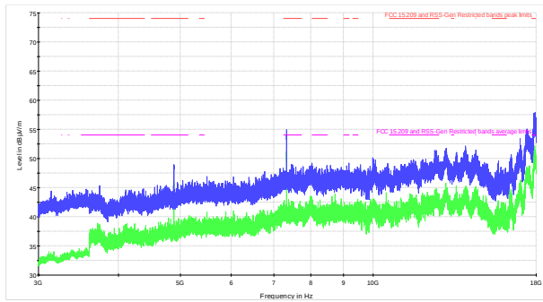
Figure 8.6-12: Conducted spurious emissions within 3–18 GHz within restricted bands, mid channel
