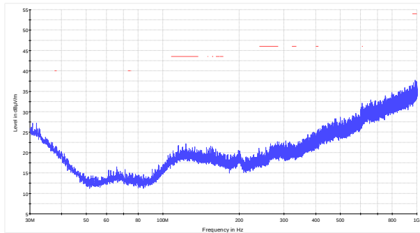
Figure 8.6-6: Radiated spurious emissions below 1 GHz within restricted bands, low channel
