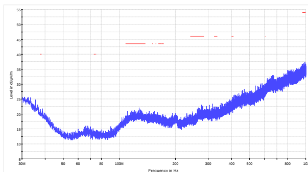
Figure 8.6-8: Radiated spurious emissions below 1 GHz within restricted bands, high channel
