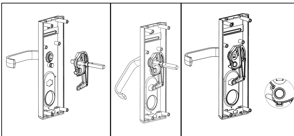
Figure D1: Handle retainer mounting instructions (this figure and Fig. D2-D3 show deadbolt below)
