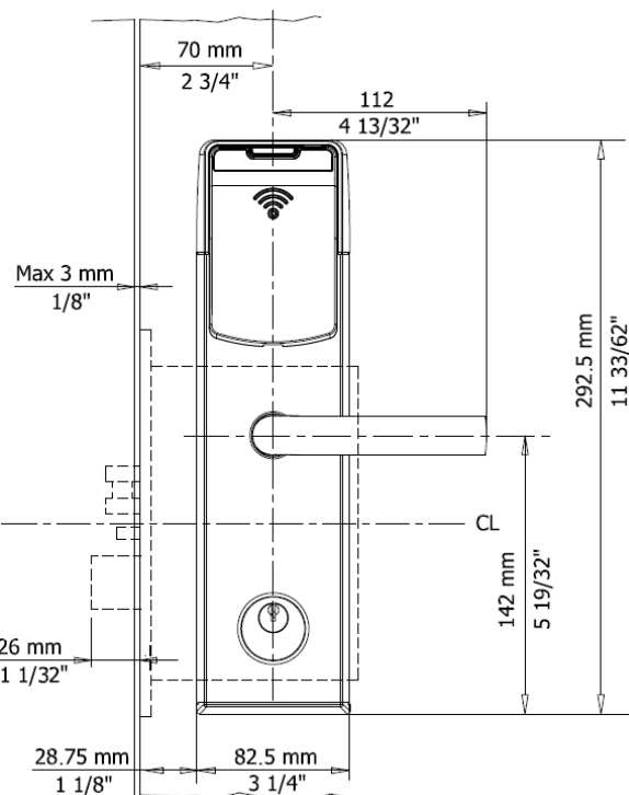
Figure 3: Escutcheon dimensions
