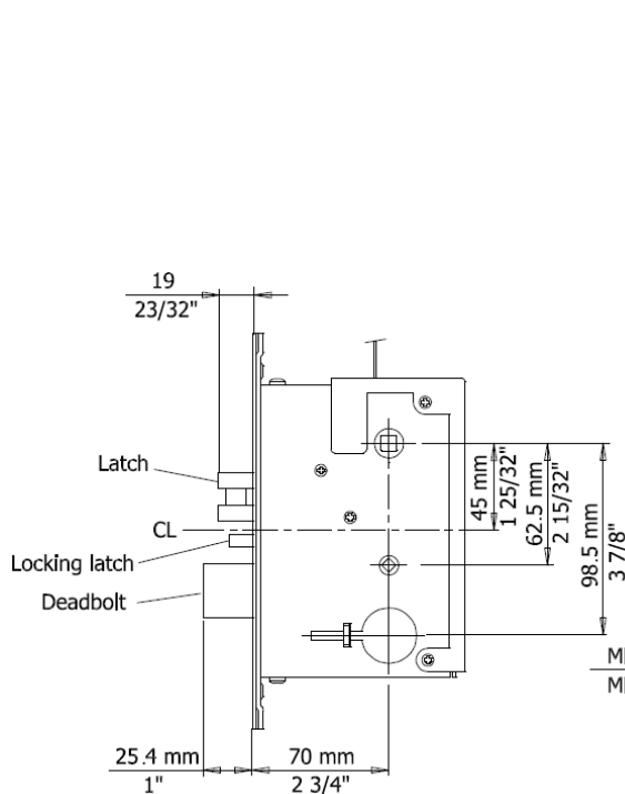
Figure 2: Lock case dimensions
