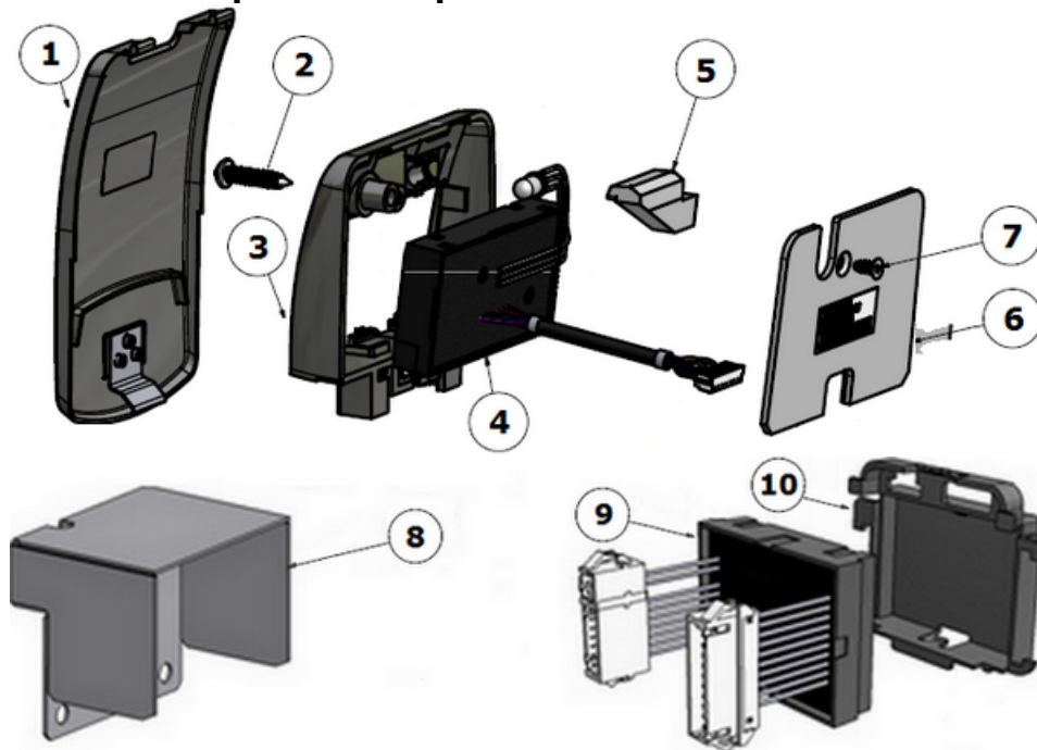
Figure 14: Note that the upgrade plate shown in pos 8 is for upgrades from Classic mag installations.
