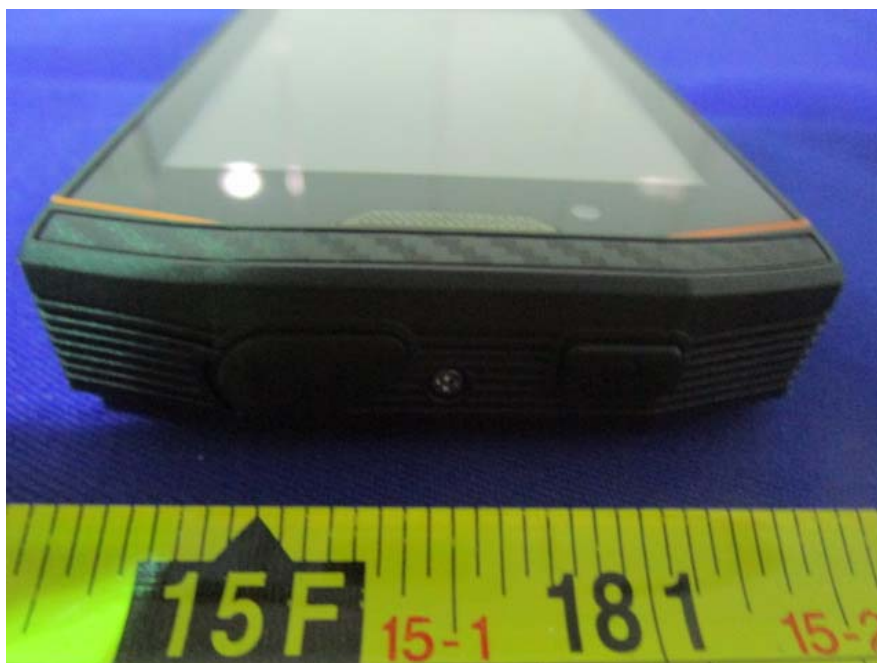
EUT – Earphone Port View
