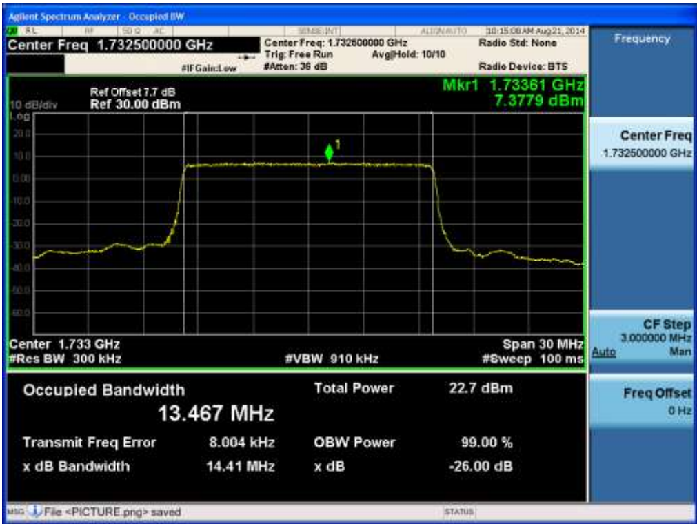
Occupied Bandwidth Plot (Band 4 – 15.0MHz 16-QAM – RB Size 75)-Middle
