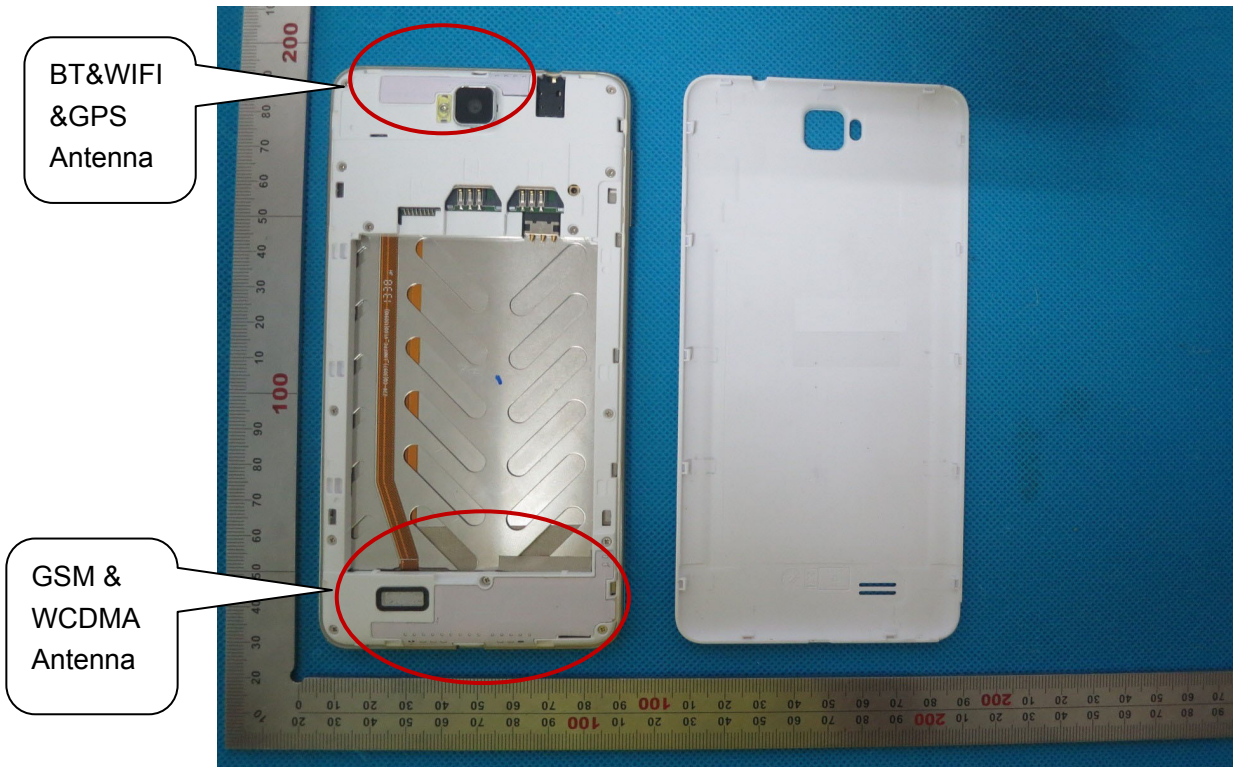
OPEN VIEW OF EUT-2
