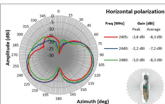
Figure 19: Radiation Pattern for XZ-Plane, Horizontal Polarization
