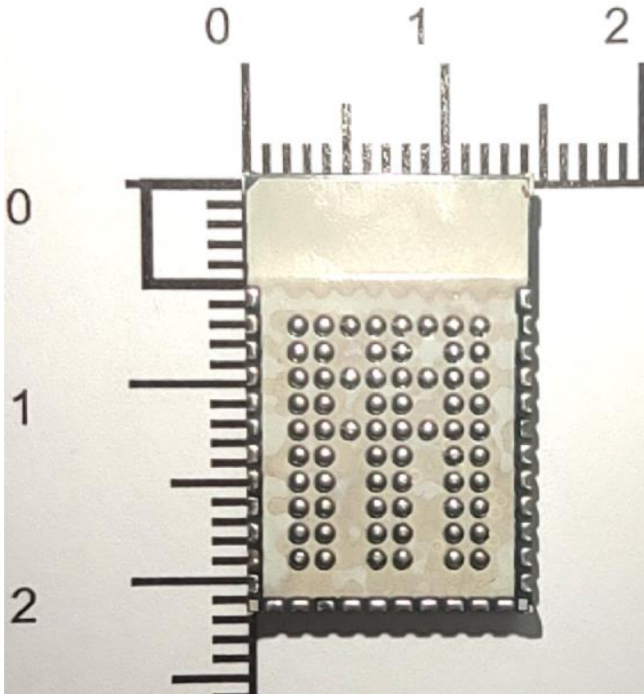
Bottom View
