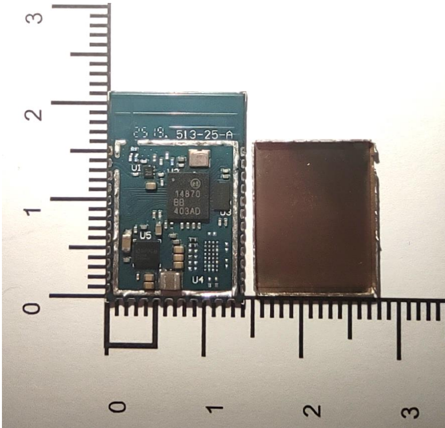
Internal circuit board photo
