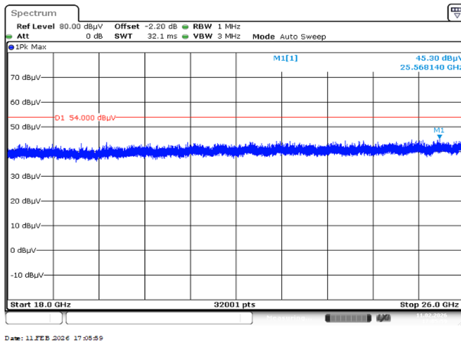
Plot 4: 18 GHz to 26 GHz, TX mode, vertical & horizontal polarization, valid for all channels and modes
